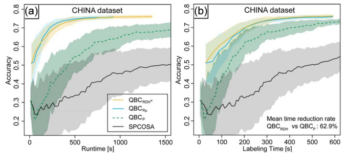
Fig. 9. Learning curves for the comparison of SPCOSA , QBC_P , QBC_{R\mu} , and QBC_{RDH}^{\times} on the China data set in terms of (a) computational runtime and (b) labeling time.
