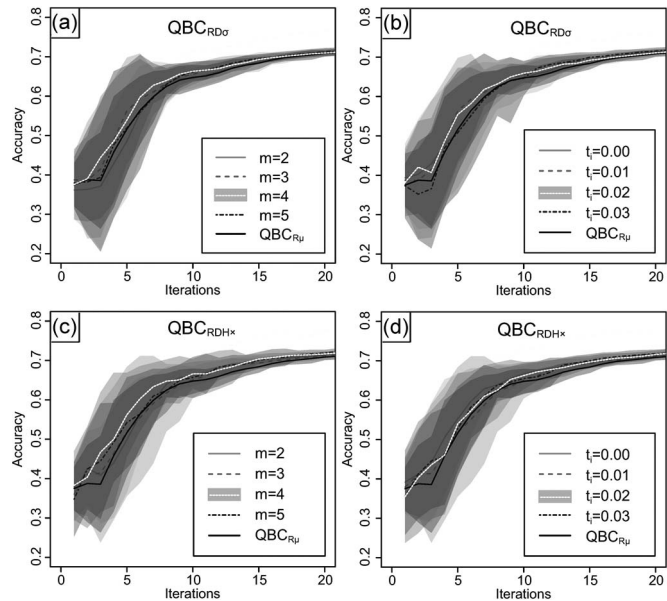
Fig. 8. Learning curves on the Brazil data set for (a) and (b) QBC_{RD\sigma} and (c) and (d) QBC_{RDH}^{\times} in dependency of changes in parameters t_i and m compared with QBC_{R\mu} at w = 100 m.
