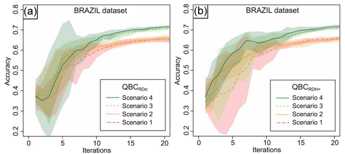
Fig. 10. Comparison of the performance of (a) QBC_{RD\sigma} and (b) QBC_{RDH}^{\times} in the four different data set scenarios for the Brazil data set.
