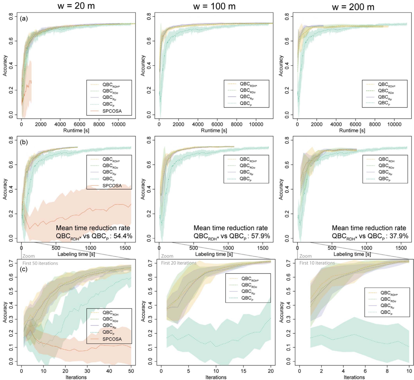
Fig. 7. Learning curves for comparison between the baseline sampling methods (SPCOSA and QBC_P ) and the proposed region-based queries ( QBC_{RD\mu} , QBC_{RD\sigma} , and QBC_{RDH}^x ) on the Brazil data set for three of the five tested window sizes. Accuracy gains are plotted with respect to (a) the computational runtime, (b) the labeling time derived by multiplying mean labeling times as detailed in Section V-A with the number of iterations, and (c) the number of iterations (early iterations, including 20 additional runs for the estimation of mean and variance). The mean time reduction rate was computed over all accuracy levels as the mean difference between the QBC_{RDH}^x -curve and the nearest corresponding points on the QBC_P -curve. For better visibility, the learning curves for SPCOSA are only presented in the first column.
