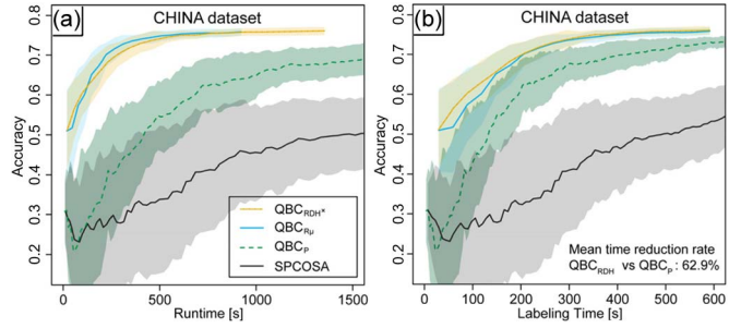
Fig. 9. Learning curves for the comparison of SPCOSA , QBC_P , QBC_{R\mu} , and QBC_{RDH}^* on the China data set in terms of (a) computational runtime and (b) labeling time.
