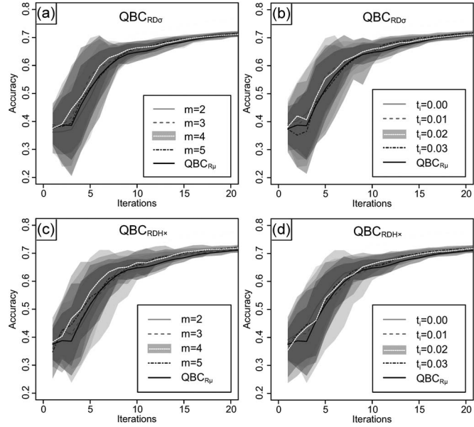
Fig. 8. Learning curves on the Brazil data set for (a) and (b) QBC_{RD\sigma} and (c) and (d) QBC_{RDH}^* in dependency of changes in parameters t_i and m compared with QBC_{R\mu} at w = 100 m.
