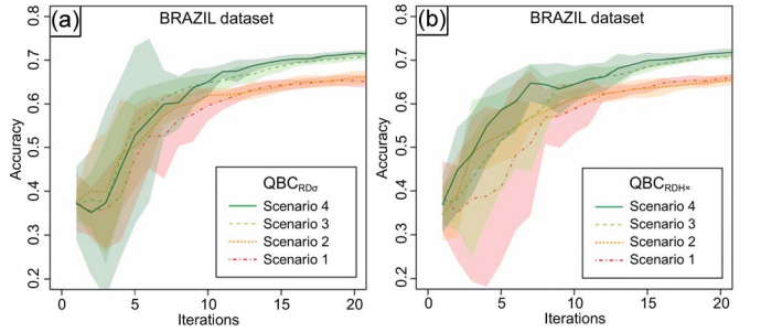
Fig. 10. Comparison of the performance of (a) QBC_{RD\sigma} and (b) QBC_{RDH}^* in the four different data set scenarios for the Brazil data set.
