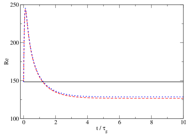
Figure 6.8: Turbulence Reynolds number Re versus time. Cases (i) solid black lines, (ii) dashed red lines, and (iii) blue dots.
