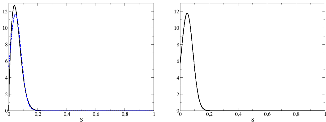
Figure 4.9: (left) Rosin Rammler distribution (dashed line) and its reconstruction by entropy maximization (solid line); (right) initial distribution given by (4.39) “close” to the Rosin Rammler distribution
