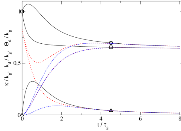
Figure 6.5: Dynamics of the normalized evaporating spray-phase energy components. Curves correspond to three initial conditions: (i) solid black lines, (ii) dashed blue lines, (iii) red dots. Curves corresponding to the fluctuating energy \kappa , the spray-phase kinetic energy k_d and the granular temperature \Theta are respectively denoted through circle, square and triangle symbols.
