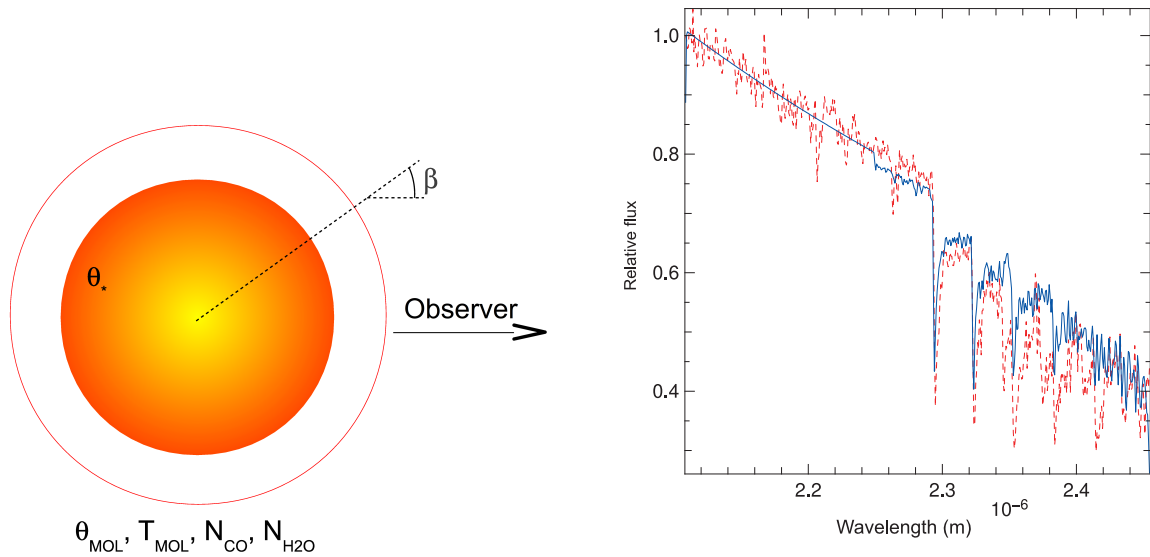
Fig. 2. Left: Illustration of the single layer model of the MOLsphere. \beta is the angle between the radius vector and the line of sight at the layer surface. Right: The red dashed line is the spectrum obtained from the Betelgeuse AMBER data and the blue continuous line is the spectrum obtained from the single layer model. We used the best fit values from Table 2.
