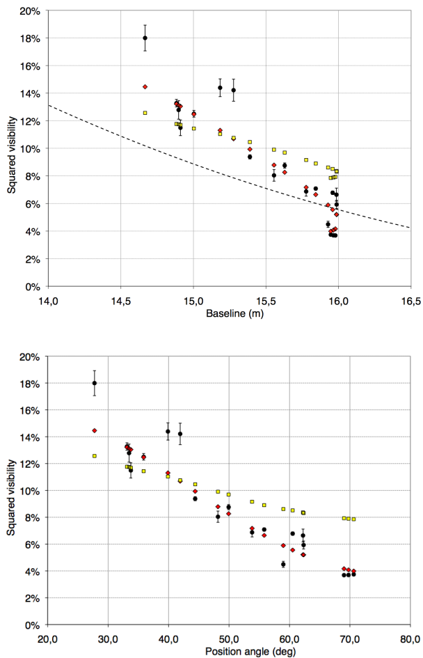
Fig. 7. VINCI squared visibilities measured on L 2 Pup, as a function of the baseline length ( top panel ) and of the baseline position angle ( bottom panel ) at an effective wavelength of 2.19 \mu\text{m} . The solid black dots are the VINCI visibility measurements, the red diamonds are the best fit uniform ellipse model visibilities (see Sect. 2.2.2 for details), and the yellow squares show the visibility derived from the RADMC-3D model presented in Sect. 3. The dashed curve in the top panel is a 26.6 mas uniform disk squared visibility function (assuming \omega = 100\% unresolved flux), intended to guide the eye.
