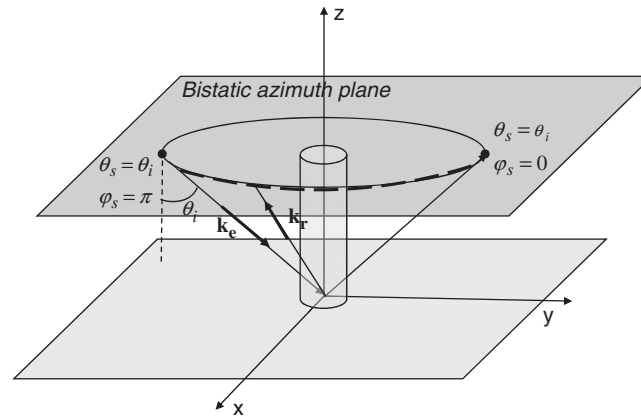
Figure 6. Configuration of measurement of one dielectric cylinder on a plate in an azimuthal bistatic configuration.
