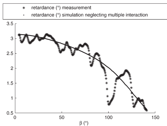
Fig. 22. Retardance parameter according to bistatic angle for a cloud of Mie spheres: results of simulation and measurement.
