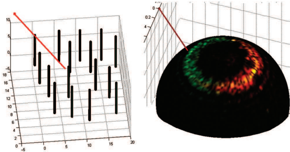
Figure 16. (Colour online) Representation on a sphere of the scattering coefficients of a group of vertical cylinders randomly located over a metallic flat surface. f=300 MHz, red: |hH+vV| , green: |hH-vV| , blue: |hV-vH| .
