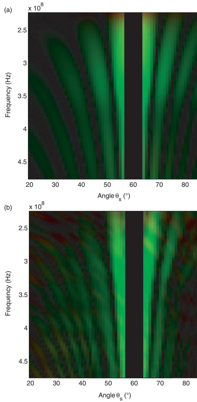
Figure 10. (Colour online) Elevation bistatic configuration: comparison between polarimetric behaviour obtained by simulation (a) and measurement (b) for one dielectric cylinder on a flat plate.
