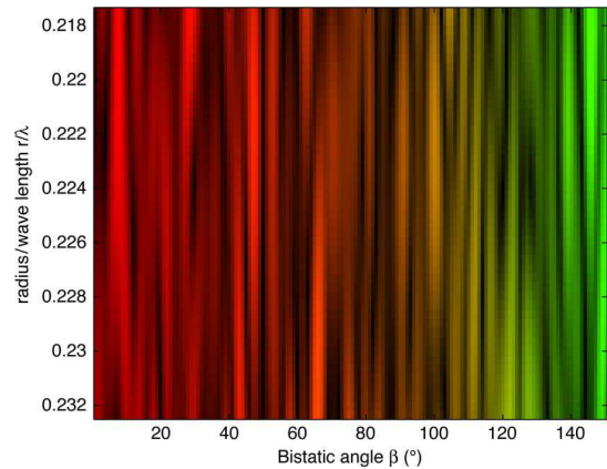
Fig. 18. Polarimetric representation of the fields scattered by a cloud of spheres according to bistatic angle and to radius/wavelength: results of simulation neglecting multiple scattering—Red: |hH + vV|^2 , Green: |hH - vV|^2 , Blue: |hV + vH|^2 .
