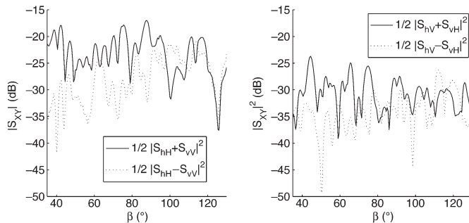
Fig. 17. Polarimetric amplitudes of the fields scattered by the cloud of spheres computed in the Pauli basis.
