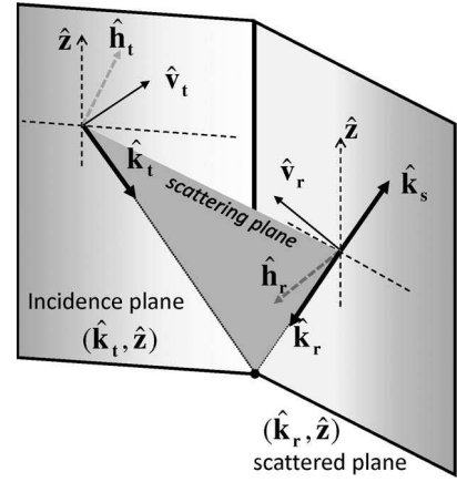
Fig. 3. Definition of the polarization vectors using the incidence and scattered planes.
