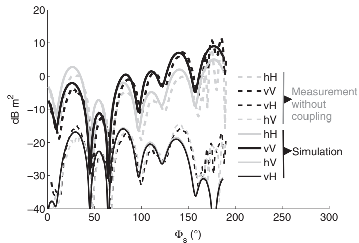
Figure 17. Comparison between the variations of the scattering coefficients for a group of three cylinders obtained by simulation and by measurement, at f=300 MHz.
