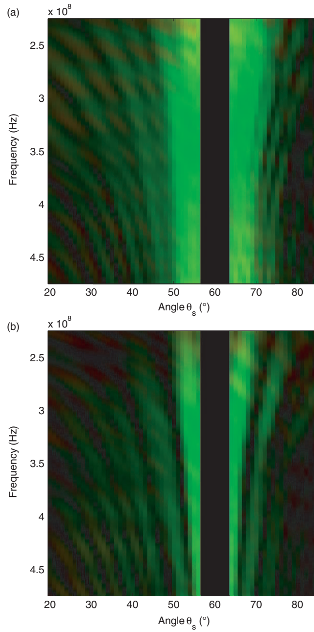
Figure 14. (Colour online) Elevation bistatic configuration: comparison between polarimetric behaviour obtained by measurement for one square cylinder (a) and a circular cylinder (b) on a flat plate.
