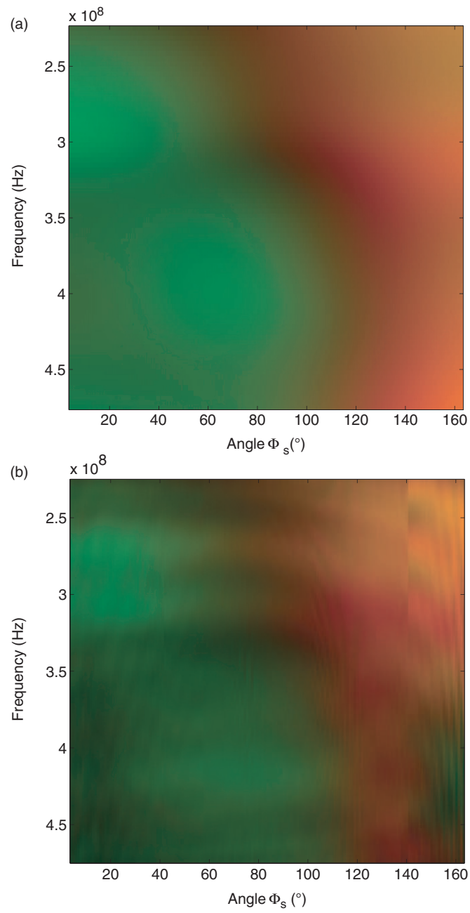
Figure 7. (Color online) Azimuthal bistatic configuration: comparison between polarimetric behaviour obtained by simulation (a) and measurement (b) for one dielectric cylinder standing on a flat plate.
