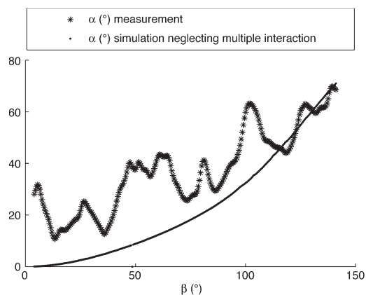
Fig. 21. \bar{\alpha} angle according to bistatic angle for a cloud of Mie spheres: results of simulation and measurement.
