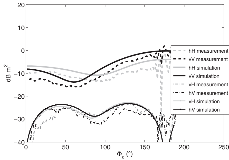
Figure 8. Azimuthal bistatic configuration: comparison between simulation and measurement of the scattering coefficients of a dielectric cylinder standing on a flat plate for all polarizations, at f=300 MHz.
