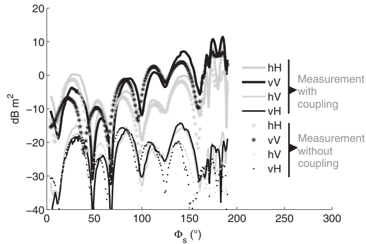
Figure 18. Comparison between two measurements of a group of three cylinders, with and without coupling, at f=300 MHz.
