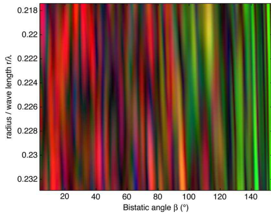
Fig. 16. Polarimetric representation of the fields scattered by a cloud of spheres according to bistatic angle and to radius/wavelength: results of measurement—Red: |hH + vV|^2 , Green: |hH - vV|^2 , Blue: |hV + vH|^2 .
