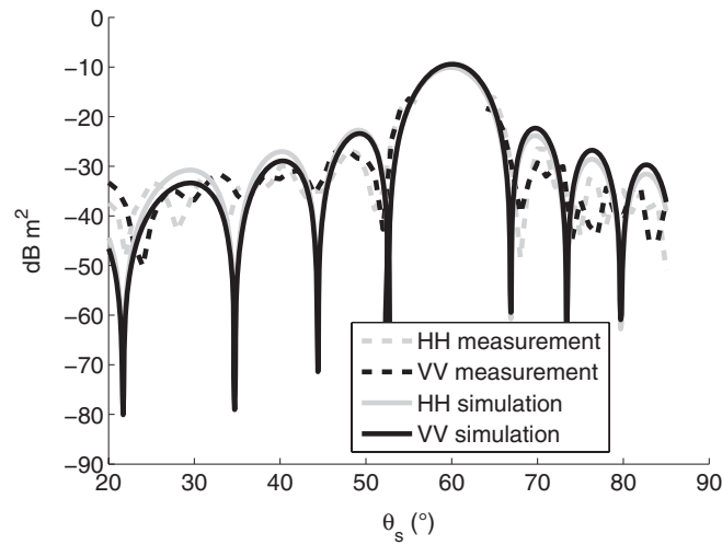
Figure 11. Elevation bistatic configuration: comparison between simulation and measurement of one dielectric cylinder on a flat plate for all polarizations at f=300 MHz.
