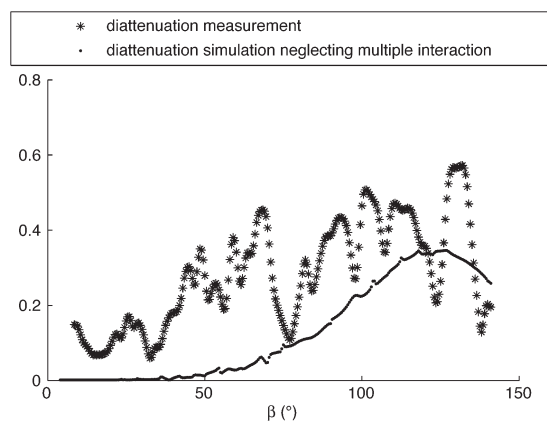
Fig. 23. Diattenuation parameter according to bistatic angle for a cloud of Mie spheres: results of simulation and measurement.
