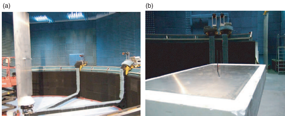
Figure 3. (Colour online) Indoor measurement capabilities for the elevation bistatic configuration (a) and the azimuthal bistatic configuration (b).
