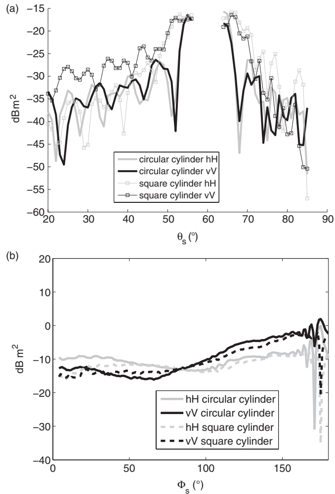
Figure 12. Comparison between the scattering coefficients of square and circular cylinders, at f=300 MHz. (a) According to the elevation bistatic angle; (b) according to the azimuthal bistatic angle.
