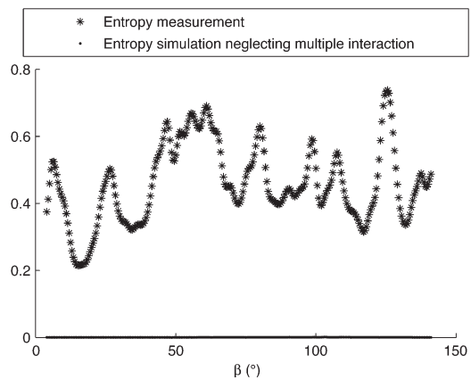
Fig. 19. Entropy parameter according to bistatic angle for a cloud of spheres in resonance region: results of simulation and measurement.
