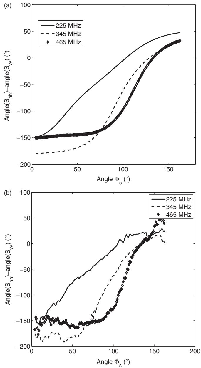
Figure 9. Phase difference between hH and vV scattered fields. (a) Simulation; (b) measurement.
