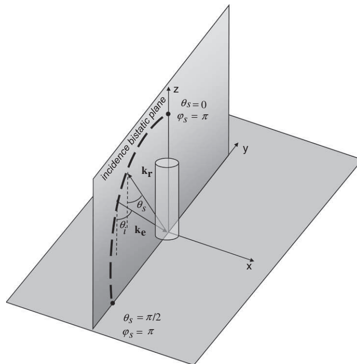
Figure 5. Configuration of measurement of one vertical dielectric cylinder standing on a plate in an elevation bistatic configuration. In this case the incidence and scattering planes are merged.
