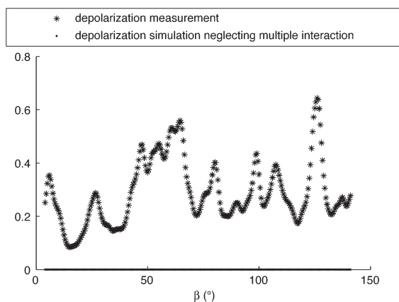
Fig. 20. Depolarization parameter according to bistatic angle for a cloud of spheres in resonance region: results of simulation and measurement.
