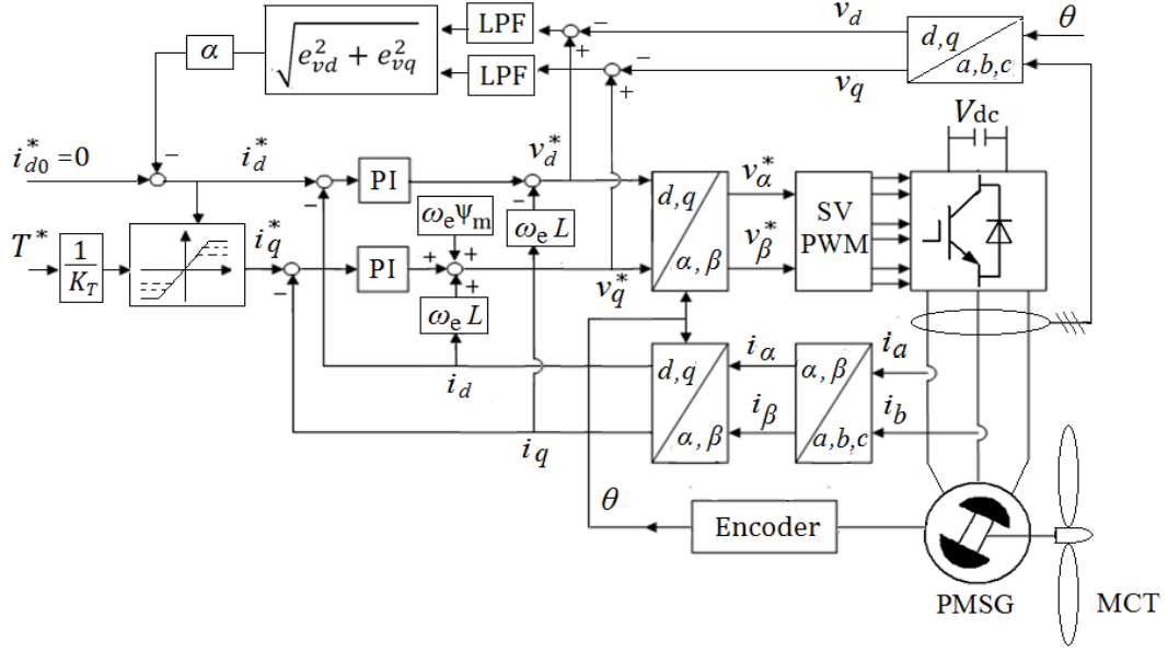
Fig. IV.5. Generator-side control scheme with flux-weakening strategy.
