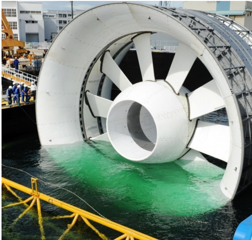
Fig. I.1. DCNS-OpenHydro turbine [12].
