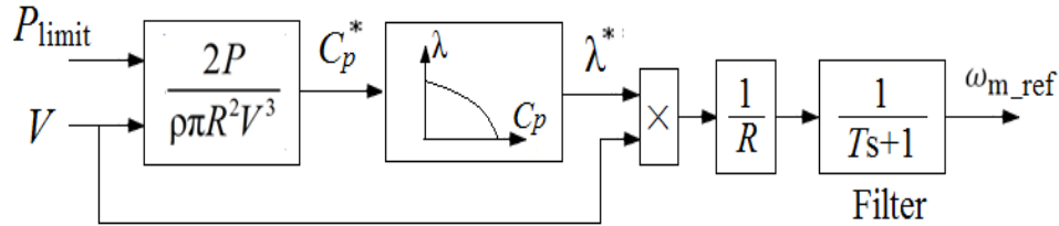
Fig. IV.6. Rotor speed reference at power limitation mode.
