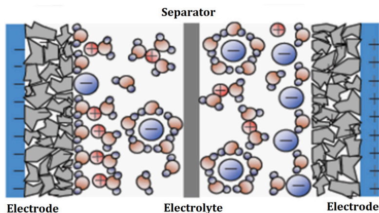
Fig. I.13. Supercapacitor cell [44].
