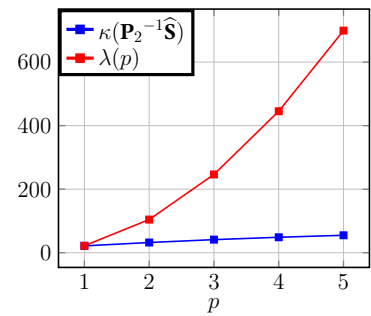
8.16.3. Preconditioner \mathbf{P}_2
