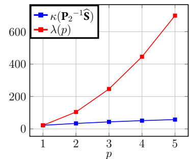
8.17.3. Preconditioner \mathbf{P}_2
