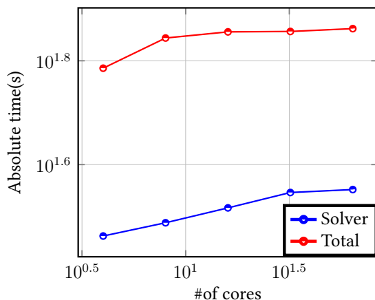
9.4.1. Absolute time versus #of cores
