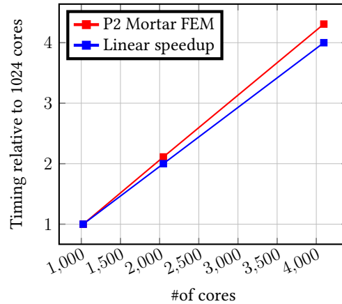
8.20.2. Second-order approximation
