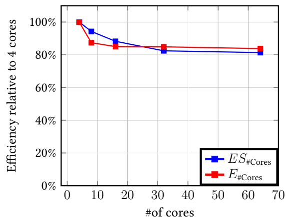
9.4.2. Efficiency versus #of cores
