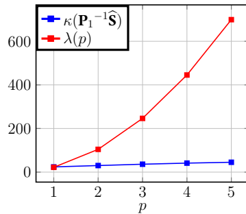
8.17.2. Preconditioner \mathbf{P}_1
