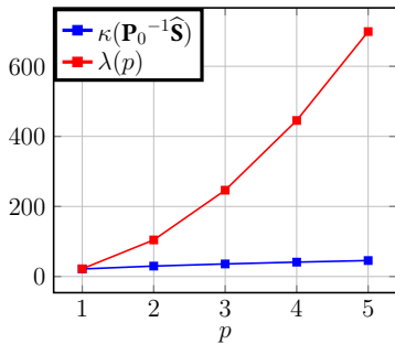
8.17.1. Preconditioner \mathbf{P}_0
