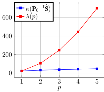
8.16.1. Preconditioner \mathbf{P}_0
