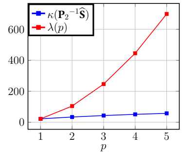
8.17.3. Preconditioner \mathbf{P}_2
