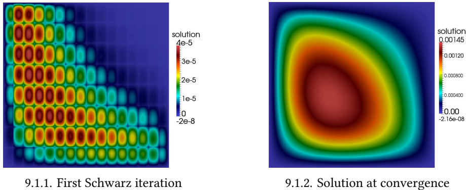
FIGURE 9.1 : Numerical solutions obtained by parallel additive Schwarz algorithm in 2D on 128 processor cores(1 subdomain/processor core)
