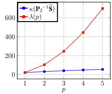
8.16.3. Preconditioner \mathbf{P}_2
