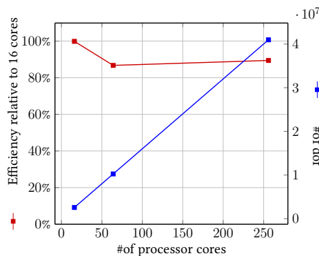
8.24.5. Fifth-order approximation
