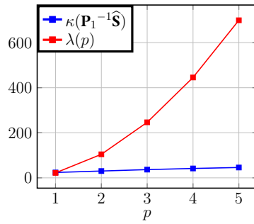
8.16.2. Preconditioner \mathbf{P}_1
