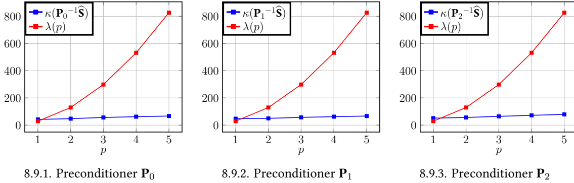
FIGURE 8.9 : \kappa(\widehat{\mathbf{P}}^{-1}\mathbf{S}) as a function of p with #of subdomains=256 and H/h = 80
