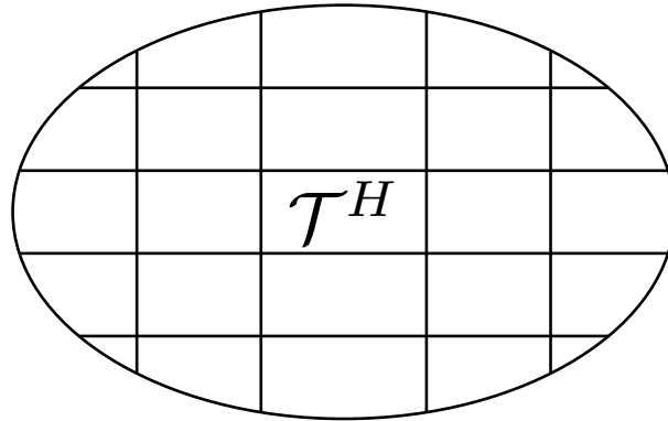
FIGURE 6.2 : Coarse mesh partition
