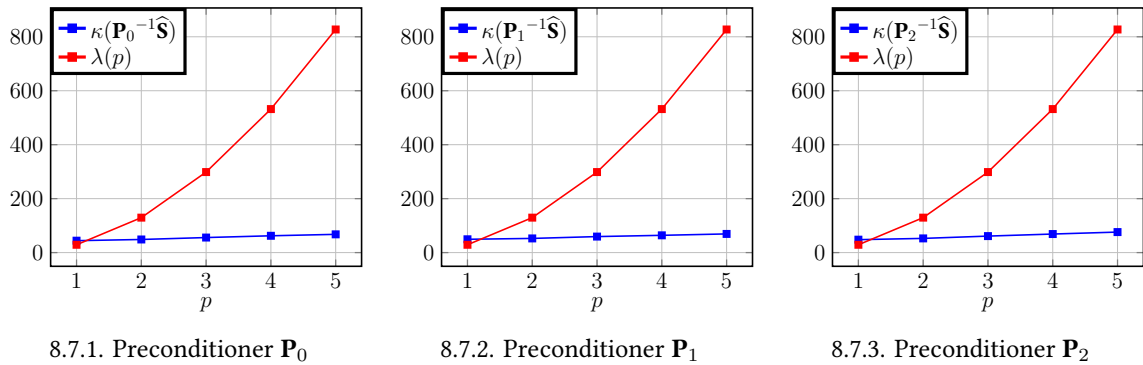
FIGURE 8.7 : \kappa(\widehat{\mathbf{P}}^{-1}\widehat{\mathbf{S}}) as a function of p with #of subdomains=16 and H/h = 80
