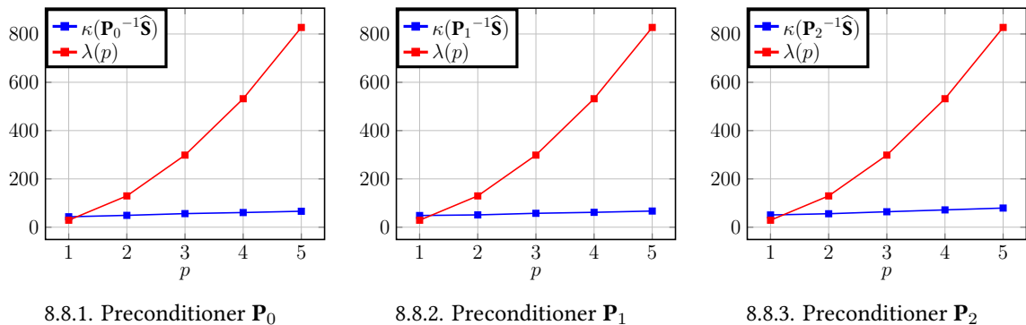
FIGURE 8.8 : \kappa(\widehat{\mathbf{P}}^{-1}\widehat{\mathbf{S}}) as a function of p with #of subdomains=64 and H/h = 80
