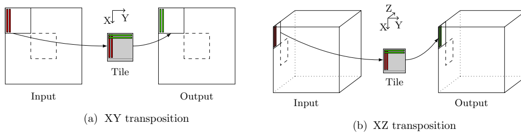
FIGURE 11. Transposition kernels.
