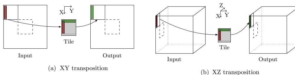
FIGURE 11. Transposition kernels.
