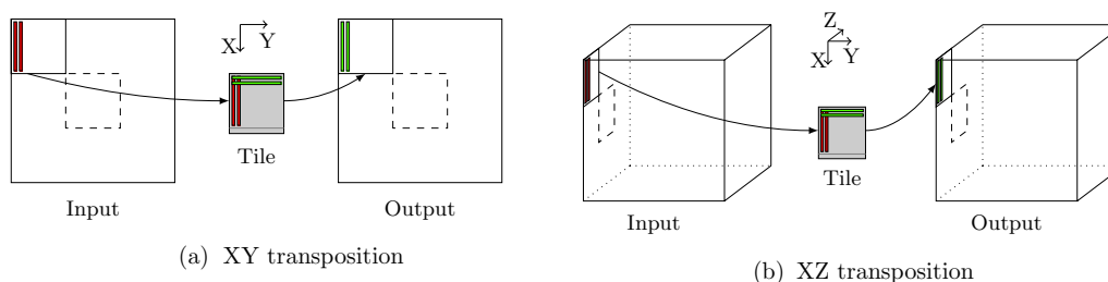
FIGURE 11. Transposition kernels.
