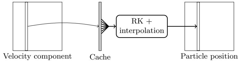
FIGURE 13. Advection algorithm.
