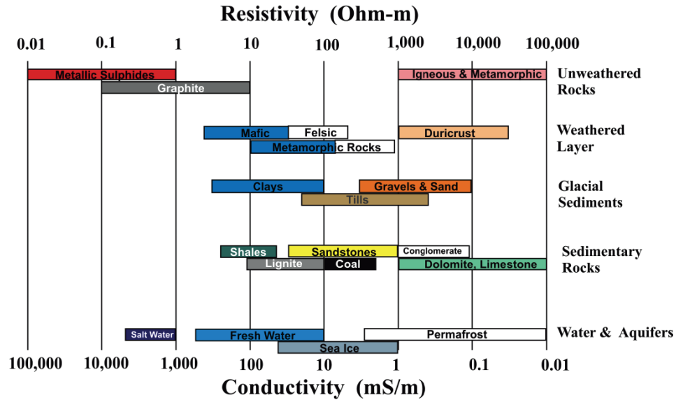
Figure 1.5: Typical electrical resistivity and conductivity values found for Earth materials. Adapted from Palacky (1988).
