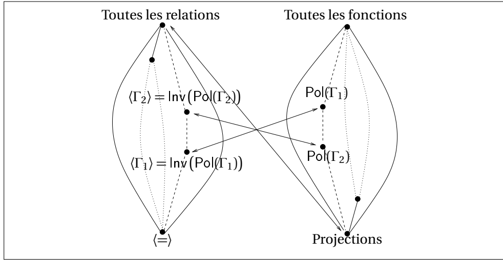
FIGURE 1.2: Correspondance de Galois Pol-Inv
