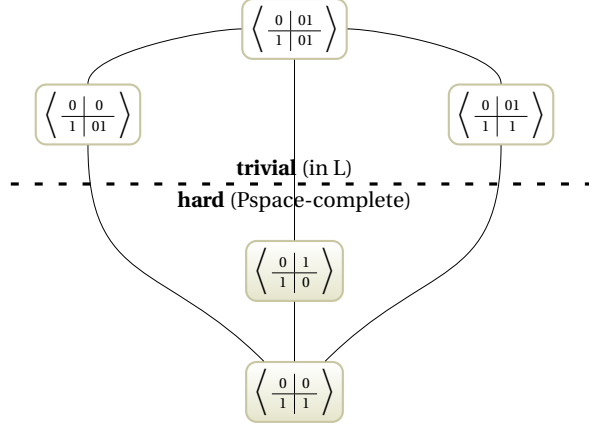
Figure 5.1: The boolean lattice of DSMs with their associated complexity.
