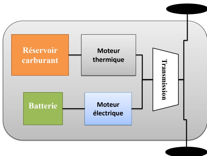
Figure I.8 – Structure mild-hybrid
