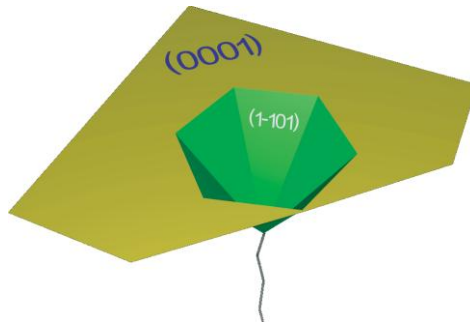
Figure 2-13: Schematic diagram of V-defects having \{1\bar{1}01\} sidewalls and emerging from the apex of a threading dislocation. 63
