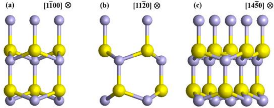
Figure 1-4: Projection of the GaN wurtzite crystal structure along a) \langle 1\bar{1}00 \rangle , b) \langle 11\bar{2}0 \rangle and c) \langle 14\bar{5}0 \rangle zone axes for a Ga polarity structure where yellow balls are for Ga atoms and the blue ones are for N atoms 3 .
