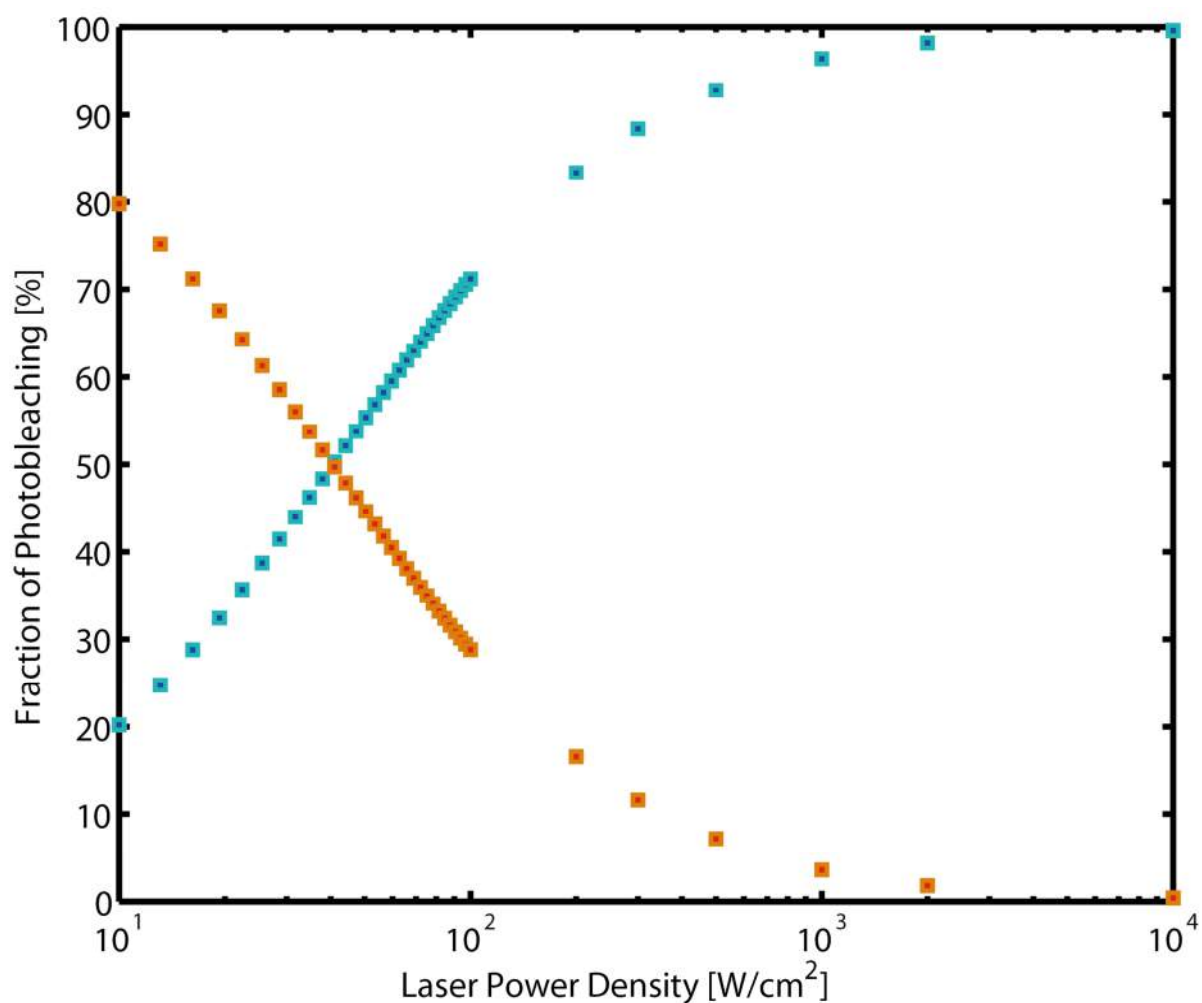
Figure S16. Power-dependence simulation of the different bleaching pathways. The fractions of photobleached protein by the respective pathways B/_{red} (blue squares) and B/_{ox} (red squares) are calculated as a function of excitation power density upon illumination for a time chosen so that 15% of molecules are bleached. Rate constants described in Figure S15 were chosen as: k_F=0.33 \times 10^9 \text{ s}^{-1} , k_{ex}=5-50 \times 10^3 \text{ s}^{-1} , k_{T1,ex}=0.15 \times k_{ex} , k_{IS}=0.3 \times 10^6 \text{ s}^{-1} , k_1=4.0 \times 10^3 \text{ s}^{-1} , k_2=3.9 \times 10^6 \text{ s}^{-1} , k_3=1.2 \times 10^5 \text{ s}^{-1} , k_{T1,1}=5.0 \times 10^3 \text{ s}^{-1} , k_{T1,2}=1.2 \times 10^6 \text{ Mol}^{-1} \text{ s}^{-1} , k_4=3.0 \times 10^4 \text{ s}^{-1} , k_5=1.0 \times 10^4 \text{ s}^{-1} , k_6=1.0 \times 10^1 \text{ s}^{-1} , k_{O2,in}=5.0 \times 10^7 \text{ Mol}^{-1} \text{ s}^{-1} , k_{O2,out}=1.0 \times 10^5 \text{ s}^{-1} with [O_2]_{medium}=200 \text{ } \mu\text{M} .
