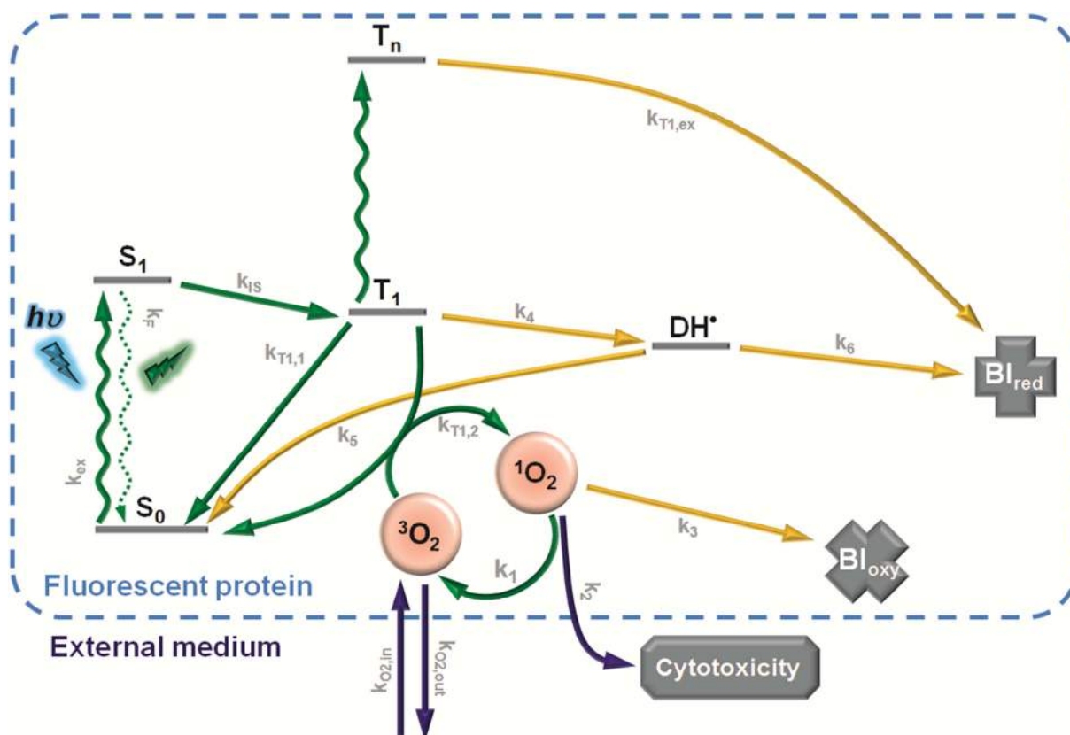
Figure S15. Putative kinetic model representative of a two-regime photobleaching in IrisFP. Description of the rate constants is provided in the SI text. Yellow arrows represent chemical steps involving e.g. electron/proton transfer or sulfoxidation reactions. Blue arrows represent entry/exit of oxygen species.
