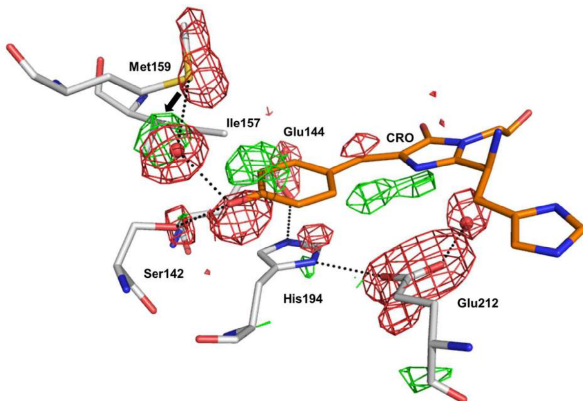
Figure S7. Structural modifications resulting from X-Ray-induced photobleaching. A NCS-averaged experimental electron difference density map is displayed. Positive density is shown in green ( +6 \sigma ) and negative density is shown in red ( -6 \sigma ), overlaid on the structure of the intact IrisFP chromophore pocket (PDB code 2VVH).
