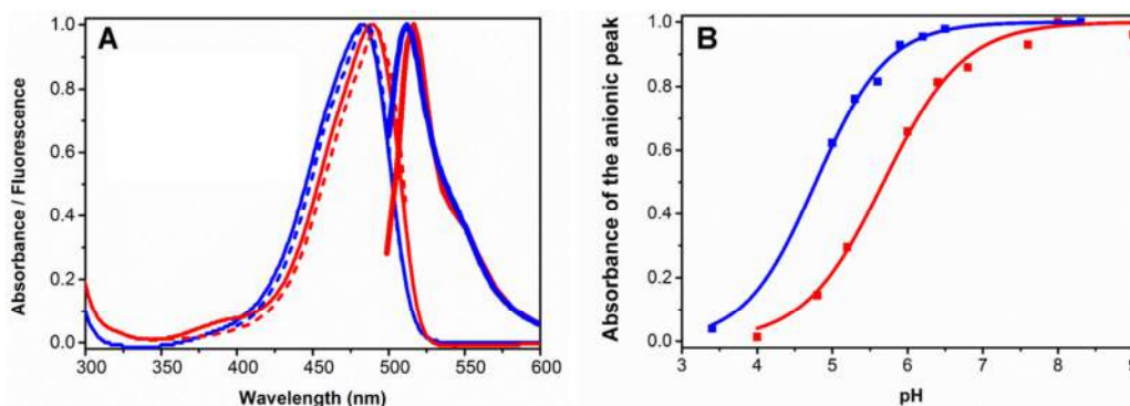
Figure 1. The mutation M159A in IrisFP only moderately affects its spectra but acidifies its chromophore. (A) Absorption (solid), excitation (dashes) and emission (bold) spectra of IrisFP (red) and IrisFP-M159A (blue) at pH 7.3. Absorption and excitation maxima peak at 488 nm for IrisFP and 484 nm for IrisFP-M159A. Emission spectra show a maximum at 516 and 513 nm for IrisFP and IrisFP-M159A, respectively. (B) Titration curves of IrisFP (red) and IrisFP-M159A (blue), demonstrating a clear acidification of the mutant's chromophore. Measurement points (squares) are fitted by the Henderson-Hasselbalch equation (lines), which yields pKa values of 5.7 for IrisFP and 4.7 for IrisFP-M159A.
