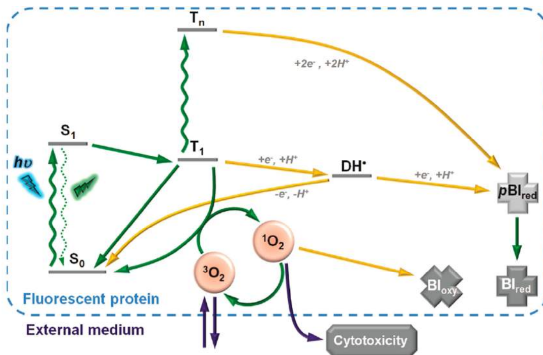
Fig15. Proposed photophysical scheme for a two-regime photobleaching in IrisFP. Yellow arrows represent chemical steps involving electron/proton transfer or oxidation reactions. Blue arrows represent entry/exit of oxygen species.
