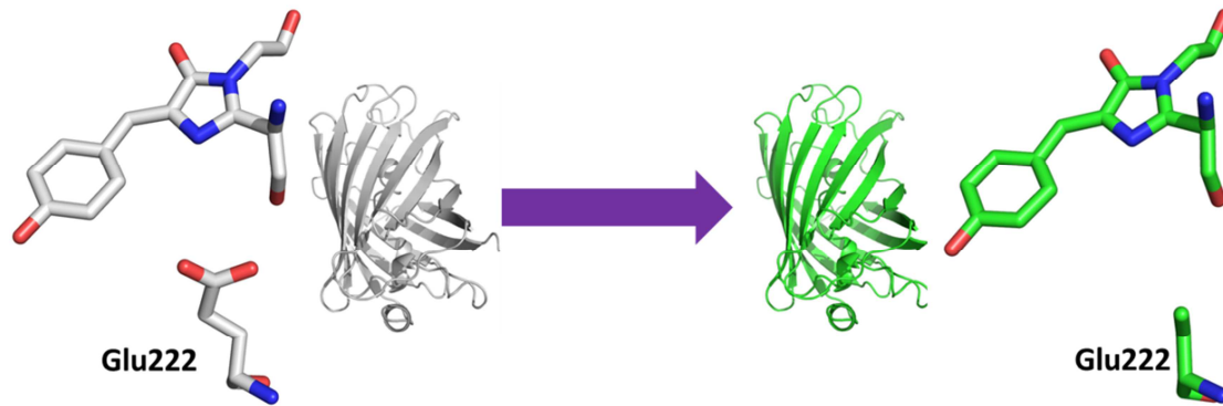
Fig5. Photoactivation of PA-GFP.
