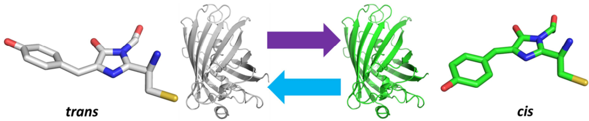
Fig7. Photoswitching of Dronpa.
