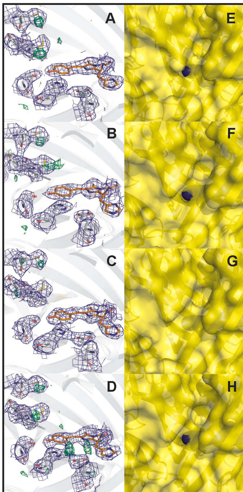
Figure S6. (A-D) Structural changes in monomers A to D induced by low-intensity photobleaching. 2F_{\text{obs}}-F_{\text{calc}} ( 1\sigma ) and F_{\text{obs}}-F_{\text{calc}} ( \pm 3.0\sigma ) electron density maps are shown as blue and green/red meshes respectively. No negative density is observed. (E-H) Surface view of monomers A to D of the IrisFP \beta -barrel. No access to the chromophore through the surface is visible in monomer C, which might explain the absence of significant sulfoxidation detected on Met159 in that monomer.
