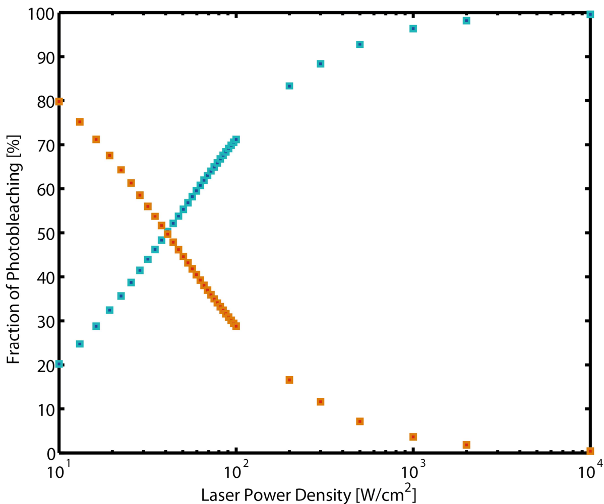
Figure S16. Power-dependence simulation of the different bleaching pathways. The fractions of photobleached protein by the respective pathways BI_{red} (blue squares) and BI_{ox} (red squares) are calculated as a function of excitation power density upon illumination for a time chosen so that 15% of molecules are bleached. Rate constants described in Figure S15 were chosen as: k_F=0.33 \times 10^9 \text{ s}^{-1} , k_{ex}=5-50 \times 10^3 \text{ s}^{-1} , k_{T1,ex}=0.15 \times k_{ex} , k_{IS}=0.3 \times 10^6 \text{ s}^{-1} , k_1=4.0 \times 10^3 \text{ s}^{-1} , k_2=3.9 \times 10^6 \text{ s}^{-1} , k_3=1.2 \times 10^5 \text{ s}^{-1} , k_{T1,1}=5.0 \times 10^3 \text{ s}^{-1} , k_{T1,2}=1.2 \times 10^6 \text{ Mol}^{-1} \text{ s}^{-1} , k_4=3.0 \times 10^4 \text{ s}^{-1} , k_5=1.0 \times 10^4 \text{ s}^{-1} , k_6=1.0 \times 10^1 \text{ s}^{-1} , k_{O2,in}=5.0 \times 10^7 \text{ Mol}^{-1} \text{ s}^{-1} , k_{O2,out}=1.0 \times 10^5 \text{ s}^{-1} with [O_2]_{medium}=200 \text{ } \mu\text{M} .
