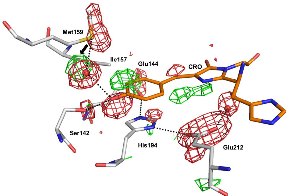
Figure S7. Structural modifications resulting from X-Ray-induced photobleaching. A NCS-averaged experimental electron difference density map is displayed. Positive density is shown in green ( +6 \sigma ) and negative density is shown in red ( -6 \sigma ), overlaid on the structure of the intact IrisFP chromophore pocket (PDB code 2VVH).
