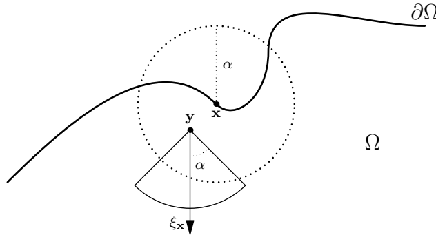
Figure 16.1: Illustration of the \alpha -cone property.
