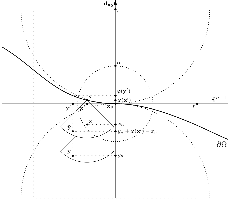
Figure 16.3: Scheme associated with the proof of Proposition 16.18.
