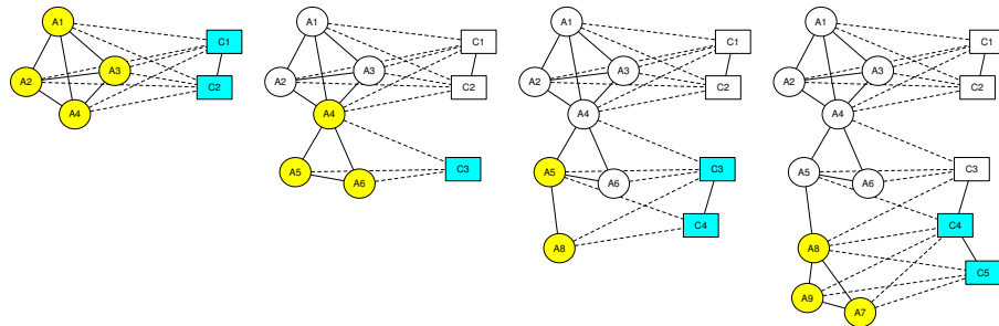
Figure 5.1: Time-evolving version of the simple example of socio-semantic network represented in Figure 4.3.
