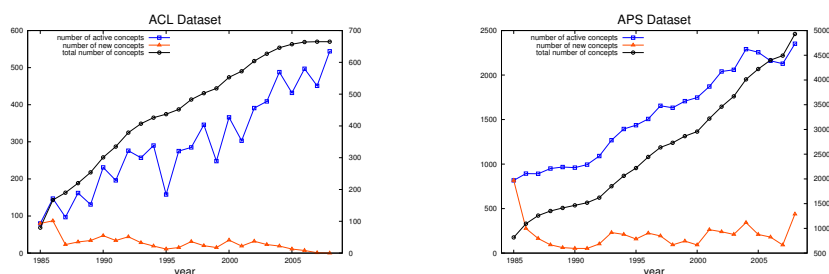
Figure 5.3: Evolution of the number of concepts over time. The scale for the black dots (i.e. the total number of concepts) is on the right y axis, whereas the scale for blue squares and orange triangles is on the left.
