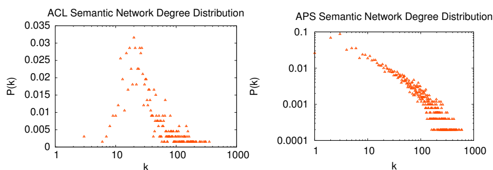
Figure 4.5: Semantic Network degree distribution, for the ACL (left) and the APS (right) data sets. Note that in the right figure both axes are in logarithmic scale, whereas in the left figure only the horizontal axis is.
