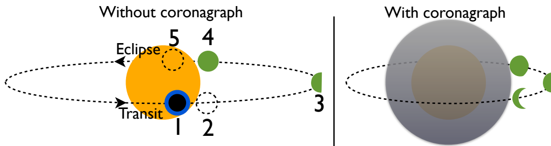
Figure I.8: Schematic of the different types of spectra of an exoplanet. The left part is the case without a coronagraph, only the total light from the star plus the planet is seen but one can have a differential spectra of the planet by comparing data from different orbital positions: (1,2) \rightarrow transit atmospheric transmission spectra, (4,5) \rightarrow eclipse reflection spectra, (2,3,4) \rightarrow phase reflection spectra (no transit nor eclipse needed). The right part is the case with a coronagraph: the star light is attenuated and the light/spectrum of the planet is observed directly.
