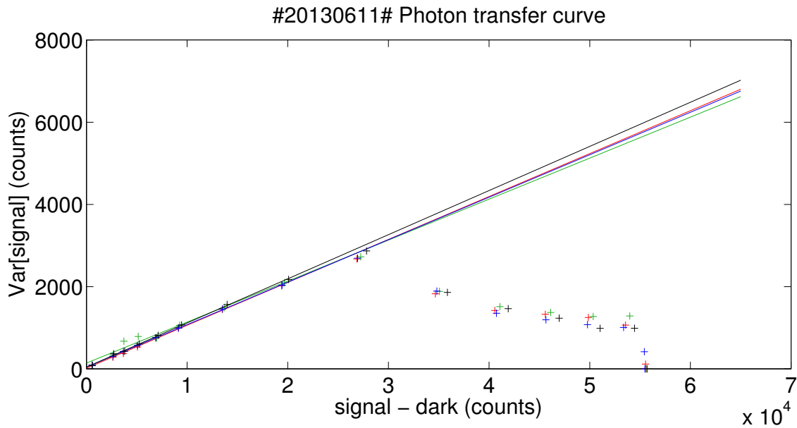
Figure III.22: Photon transfer curve: \sigma_S^2 vs. S - S_{\text{offset}} (Set 1: 11/06/2013). The Framerate is 100 Hz.
