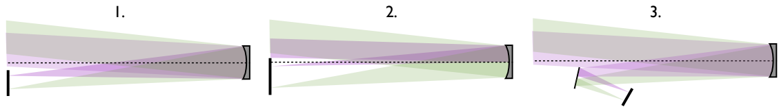
Figure II.5: Illustration of the “beam walk” problem (term coined by Mike Shao). Configuration 1 is NEAT-like, there is no obscuration. Configuration 2 has some obscuration on part of the field: the purple beam footprint is only half of the mirror and is affected by different systematic errors than the green one. Configuration 3 has two mirrors: the beams have not the same footprint on the secondary mirror, they are also affected by different systematic errors. A TMA configuration with a central obscuration by the secondary would suffer from the issues of configurations 2 and 3.
