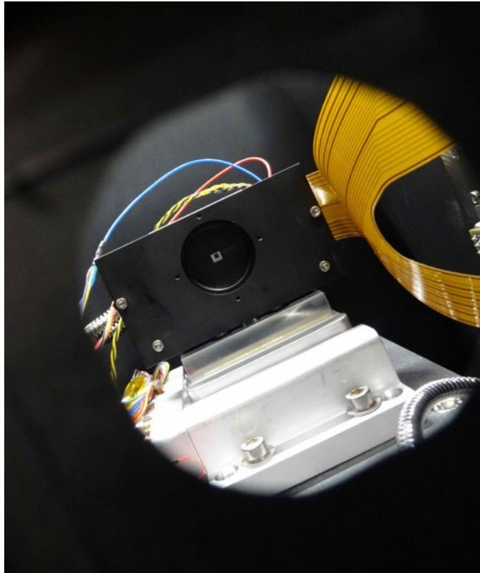
Figure III.13: Baffle v2. The picture is taken in front of the chip, just behind the outer vane inside the vacuum chamber. The small square inside the bright area is the sensitive area of the chip. The black square around the bright area next to the chip is the inner vane.
