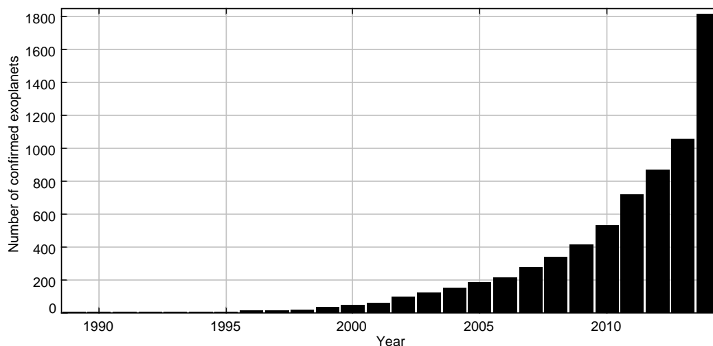
Figure I.1: Cumulative histogram of the number of confirmed exoplanets, sorted by year of discovery, from 1989 to 2014 (Credit: exoplanet.eu database, updated: 12/07/2014). The histogram starts before 1992 because the database includes a prior discovery [Latham et al., 1989] of an object with a high and uncertain mass, it could be a planet or a very low mass star depending on the orientation of the orbit, see radial velocities in section 1.2.1 for detailed explanations. The high number of new exoplanets in 2014 comes from the Kepler mission [Rowe et al., 2014].
