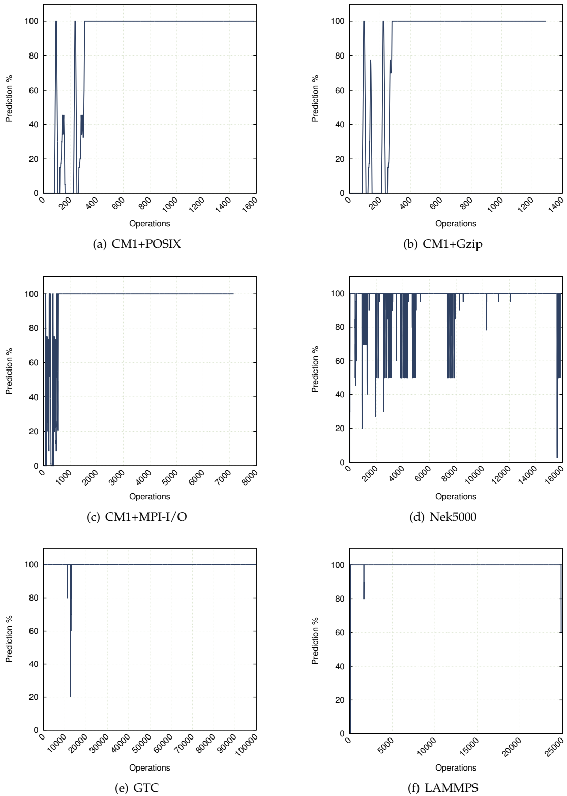
Figure 7.2: Context prediction capability of Omnisc'IO over the run of each application. Configurations (a), (b), (c), (e), and (f) exhibit a clear learning phase after which Omnisc'IO makes perfect predictions ((e) and (f) exhibit a drop of prediction at the end of the first iteration).
