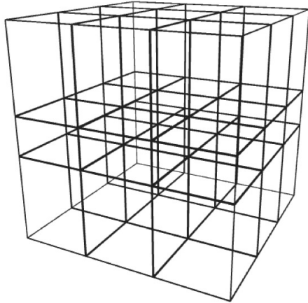
Figure 4.2: Example of a 4 \times 4 \times 4 rectilinear grid described by three arrays of coordinates. In this example there is a scalar value (such as temperature or wind velocity ) at each node. The mesh itself is described through three coordinate arrays: mesh_x = {0.0,1.0,2.0,3.0} ; mesh_y = {0.0,1.0,2.0,3.0} ; mesh_z = {0.0,1.2,1.8,3.0} .
