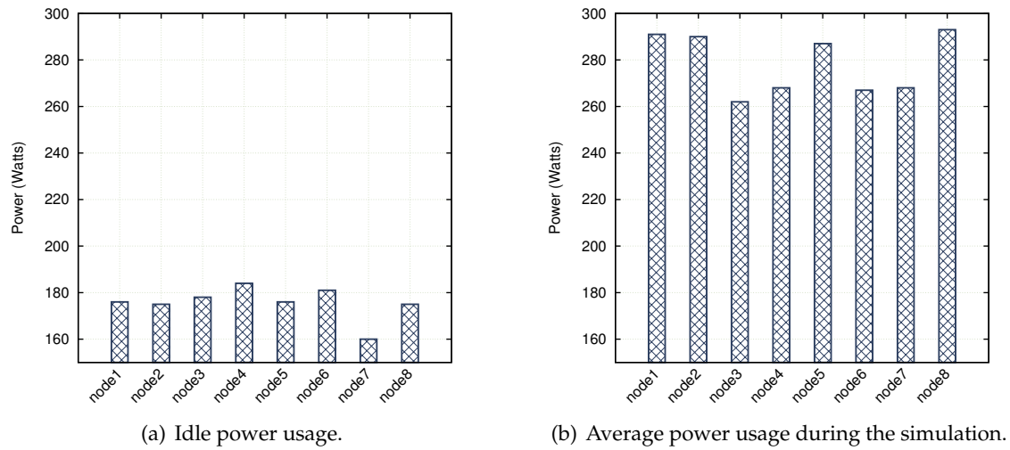
Figure 5.9: Power usage of the paraplue cluster of Grid'5000 when the nodes are idle and when they run the simulation
