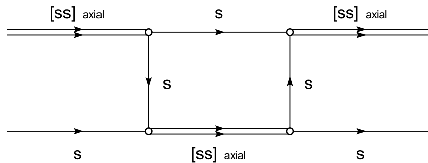
Figure 16. Baryon \Omega^- .
