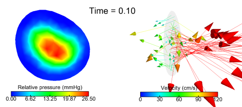
Figure 5.5: In-plane pressure gradient (left) and velocity fields (right) at the LPA interface during maximal forward flow ( t=0.1 s) with the 3D-0D-Ptot coupling method.
