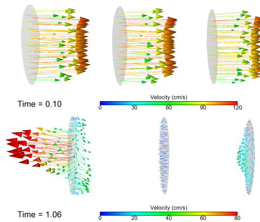
Figure 5.4: Velocity fields at the LPA interface, when flow at the inlet is maximal forward (top, t=0.10 s, Q_{\max} = 378 \text{ cm}^3/\text{s} ) and is reverse (bottom, t=1.06 s, Q_{\min} = -66 \text{ cm}^3/\text{s} ) with the 3D-0D , 3D-0D-Stab and 3D-3D coupling methods from left to right.
