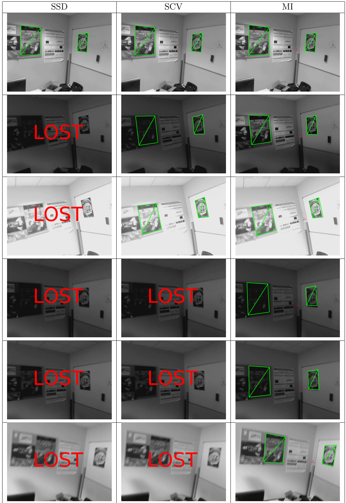
Figure 3.9: Results of the SSD (on the left), SCV (in the middle) and MI (on the right) model-based algorithms in light varying conditions. The SSD is lost at the first light variation, whereas light variations do no impact the SCV but it is still lost when too much blur appears in the image.
