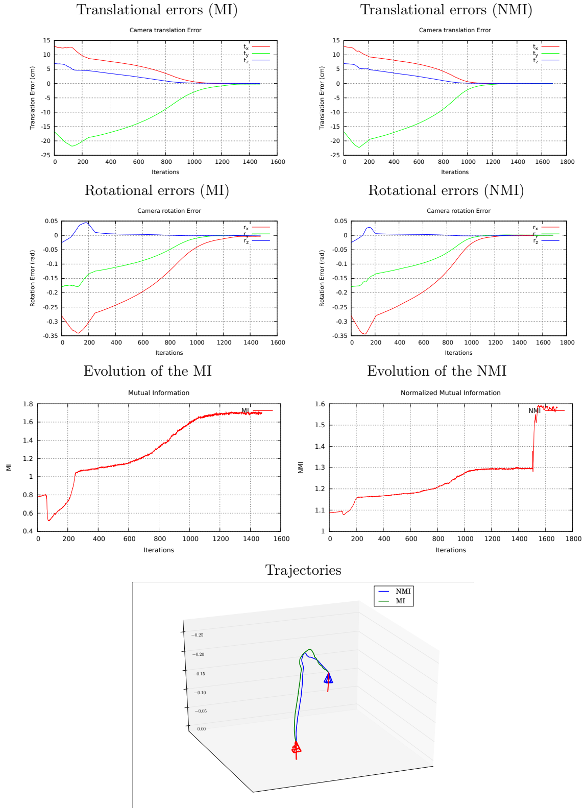
Figure 7.5: Comparison of NMI and MI-based visual servoing methods in light varying conditions.
