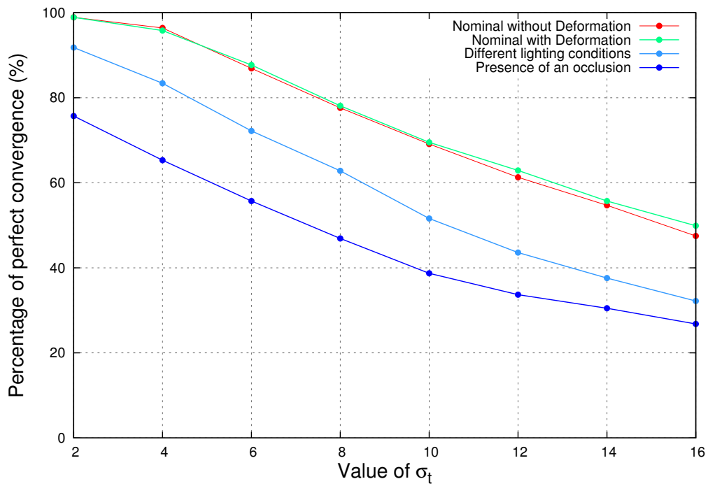
Figure 4.13: Convergence frequency of the MI approach in nominal conditions without deformation (row 1 of fig. 4.11), with deformations (row 2 of fig. 4.11), when confronted to light variations (row 3 of fig. 4.11) and when confronted to occlusions (row 4 of fig. 4.11).
