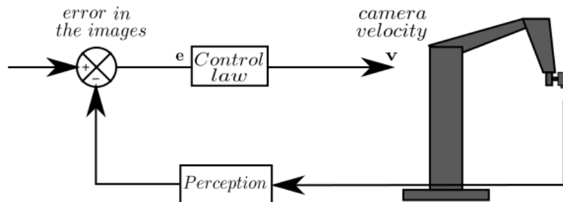
Figure 5.1: Classical visual servoing loop. The perception allows to evaluate a task \mathbf{e} in order to compute a camera velocity \mathbf{v} . The robot is controlled according to a comparison between the desired and perceives visual data.
