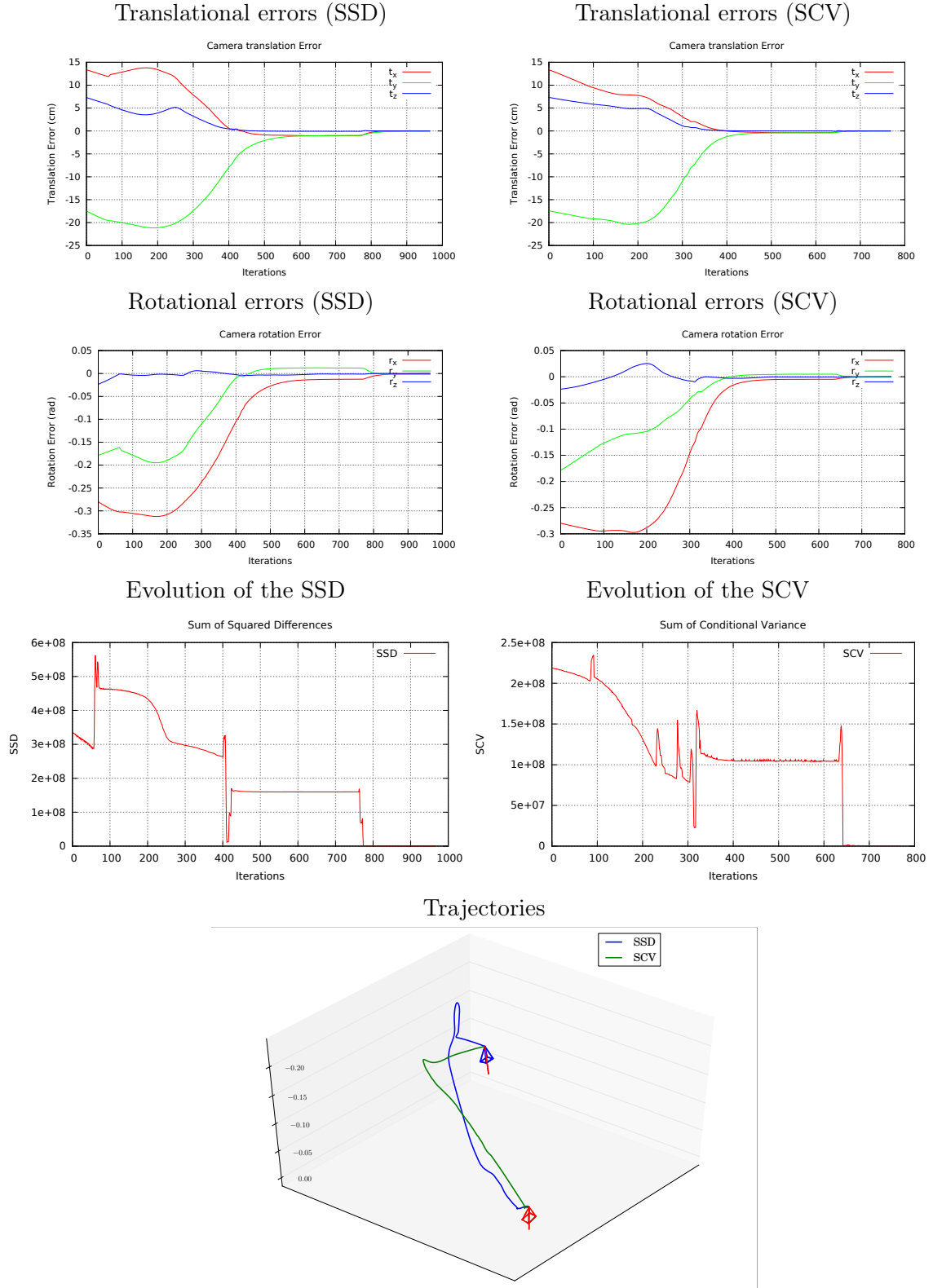
Figure 6.11: Comparison of SCV and SSD-based visual servoing methods in the presence of occlusions.
