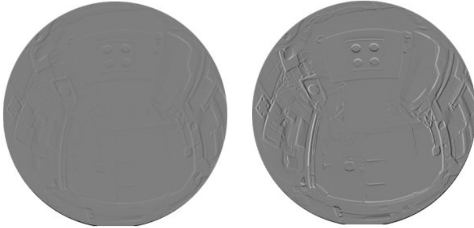
Figure 7.10: From left to right: Gradient image computed on the image plane and gradient image computed from the equivalence sphere. [Caron et al., 2010]
