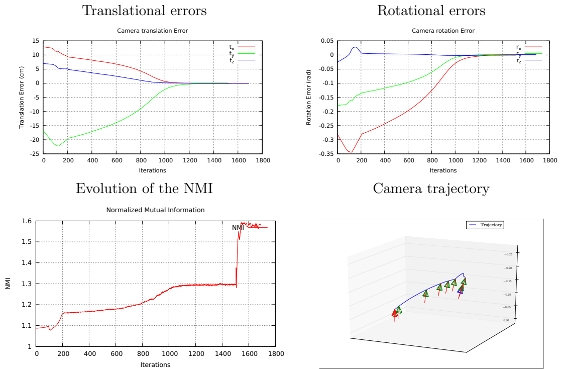
Figure 7.4: Results of NMI-based visual servoing in light varying conditions.
