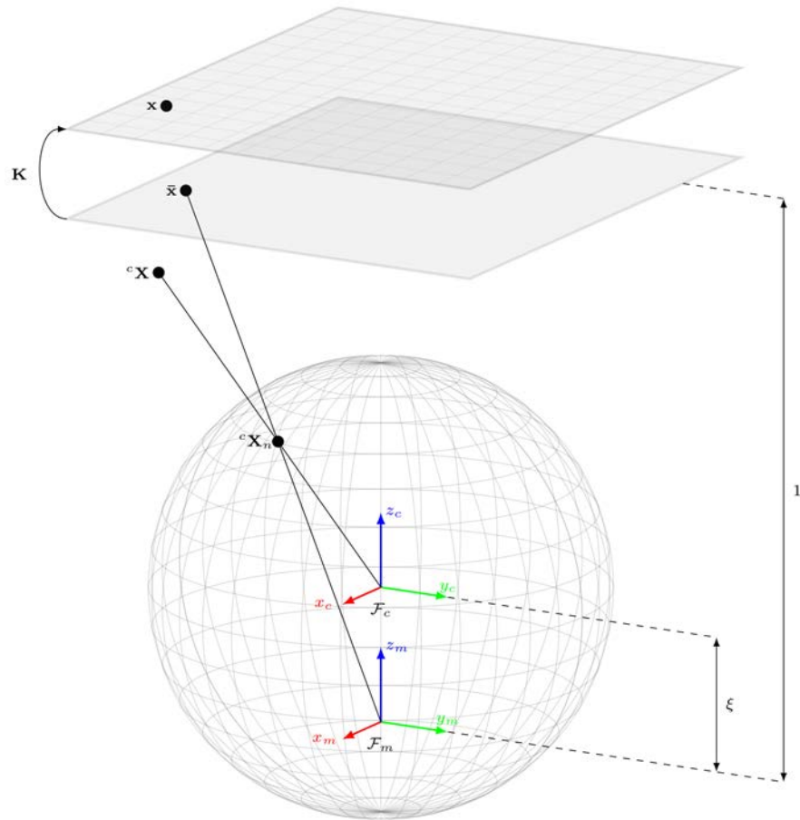
Figure 7.9: Illustration of the unified projection model (proposed with the authorization of [Markovic et al., 2014]). Full pipeline of projection from a 3D point {}^c\mathbf{X} to a point \mathbf{x} in the image.
