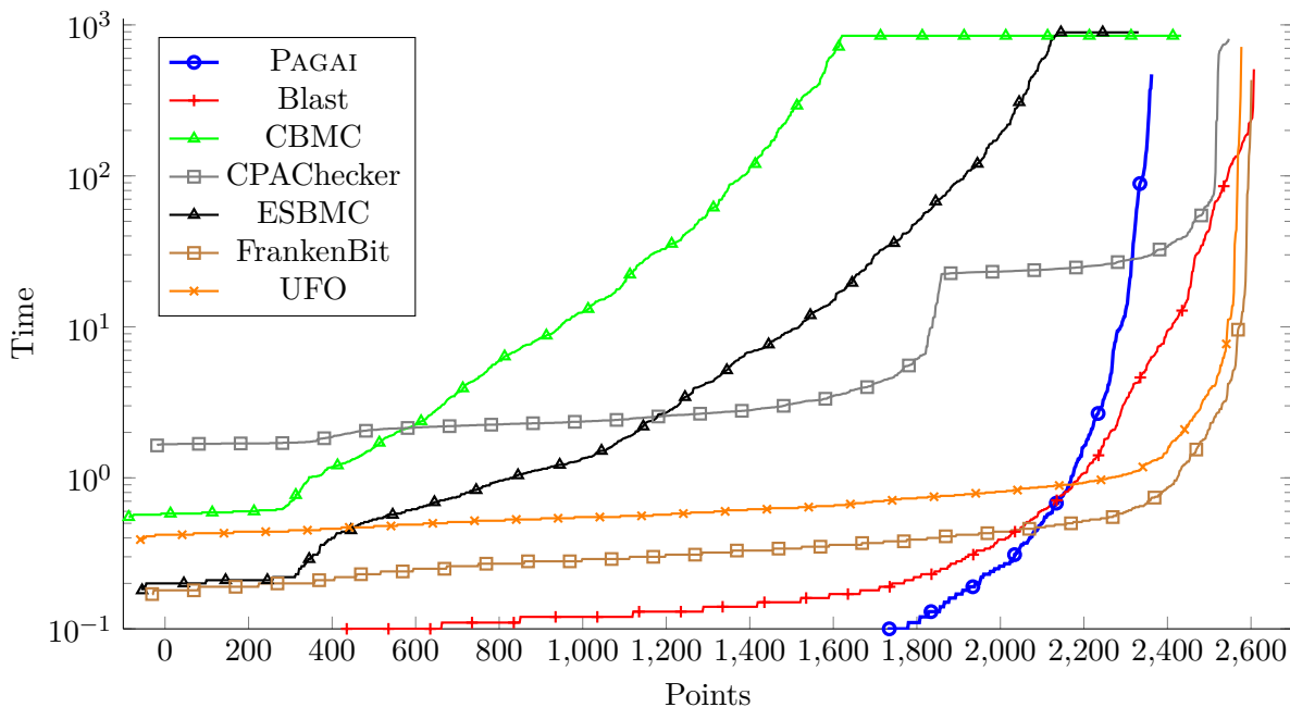
Figure 7.15: Category DeviceDrivers64, TRUE benchmarks
