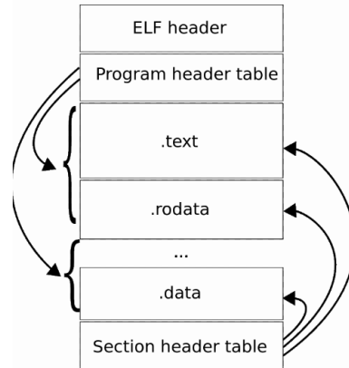
Figure 9.13: ELF executable layout.
