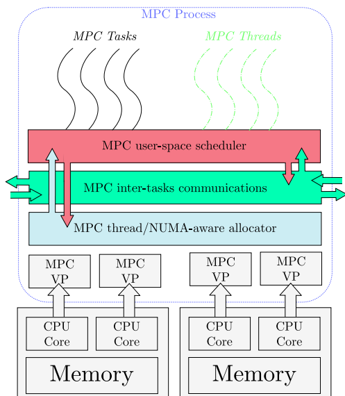
Figure 1.1: Overview of the MPC runtime.
