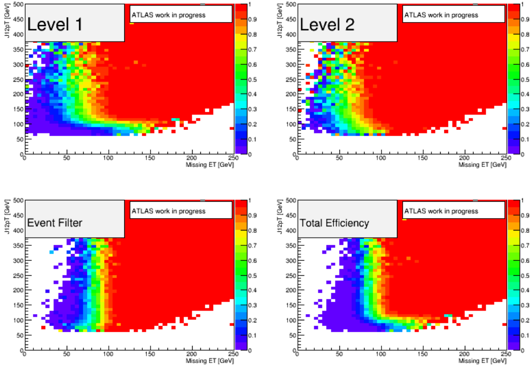
Figure 4.24: E_T^{\text{miss}} trigger turn-on dependence with respect to J12pT for trigger EF_xe80_tclw_loose for Z \rightarrow \mu\mu sample in 2-jet bin on MC. The colors correspond to the efficiency.
