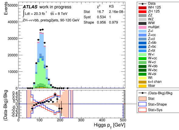
Figure 5.14: Distribution of Higgs boson p_T using delayed stream trigger inclusively in region 90 < E_T^{\text{miss}} < 120 GeV.
