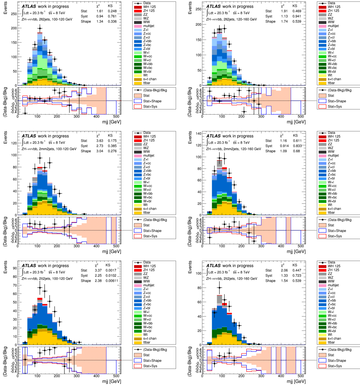
Figure 5.17: Distribution of invariant mass of two b -jets for LL, MM and TT tag regions (in 2-jet bin and in 2 bins of E_T^{miss} : 100–120 GeV and 120–160 GeV) of b -tagging category of the analysis using delayed stream trigger (pre-fit).
