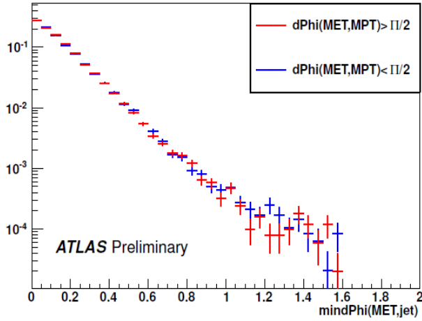
Figure 5.8: Distribution of \min \Delta\phi(E_T^{\text{miss}}, jets) of multijet background in region of \Delta\phi(E_T^{\text{miss}}, P_T^{\text{miss}}) < \pi/2 (blue) and \Delta\phi(E_T^{\text{miss}}, P_T^{\text{miss}}) > \pi/2 (red) using data [101]. This distribution is made in region of first E_T^{\text{miss}} bin, before applying b -tagging.
