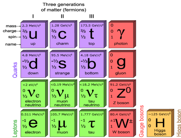
Figure 1.2: Particle hierarchy in Standard Model with their characteristics.
