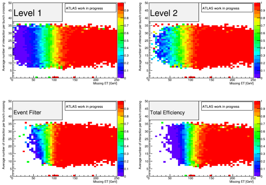
Figure 4.20: E_T^{\text{miss}} trigger turn-on dependence with respect to the average number of interactions per bunch crossing for trigger EF_xe80_tlcw_loose for Z \rightarrow \mu\mu sample in 2-jet bin (on data). The colors correspond to the efficiency.
