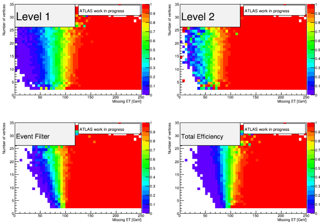
Figure 4.18: E_T^{\text{miss}} trigger turn-on dependence with respect to number of vertices for trigger EF_xe80_tclw_loose for Z \rightarrow \mu\mu sample in 2-jet bin on MC samples. The colors correspond to the efficiency.
