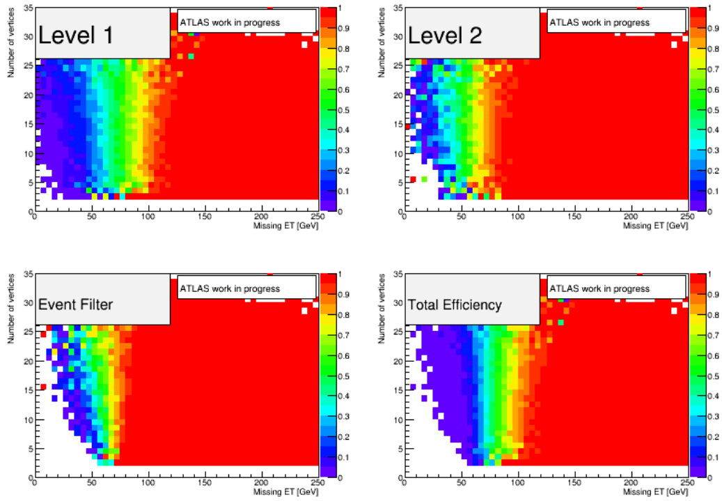
Figure 4.19: E_T^{\text{miss}} trigger turn-on dependence with respect to number of vertices for trigger EF_xe60_tlcw_loose_delayed for Z \rightarrow \mu\mu sample in 2-jet bin on MC samples. The colors correspond to the efficiency.
