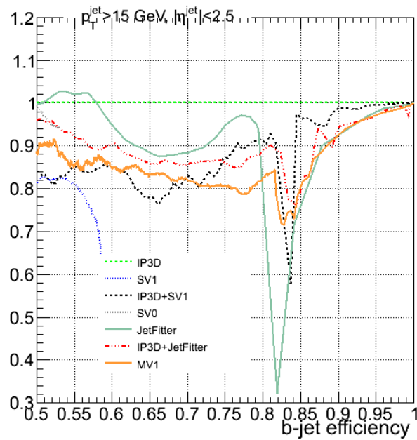
Figure 3.24: Ratio of b -tagging performance for ghost-association jets, the numerator is the performance for p_T of ghost-association with p_T > 1.5 \text{ GeV} for track selection, and the denominator is before applying this modification ( p_T > 1 \text{ GeV} ). The modification of p_T > 1.5 \text{ GeV} on the IP-based selection is applied.
