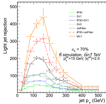
Figure 3.12: Light jet rejection as function of jet transverse momentum p_T for b -tagging efficiency \epsilon_b = 70\% , based on simulated t\bar{t} events.
