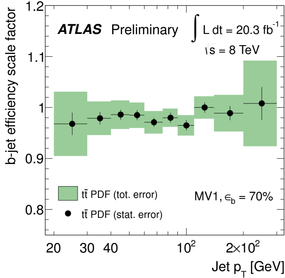
Figure 3.25: The b -tagging efficiency scale factor of data-to-MC for the b -tagging algorithm MV1 with 70% of b -tagging efficiency using t\bar{t} events at each bin of p_T of jet. The green band represents the total uncertainty of the combination of the two methods [70].
