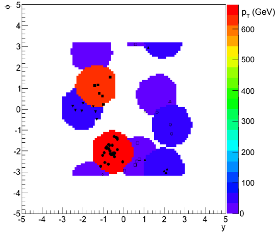
Figure 3.4: Event display in y/\phi plane showing anti- k_t jets with \Delta R = 1 and displaying the use of ghost tracking. Different pattern marks (open or plain circles, triangles, etc...) correspond to tracks belonging to different jets, the colors correspond to p_T of jets.
