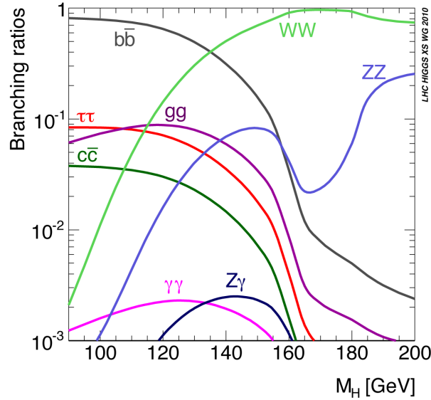
Figure 1.9: Branching ratio of each decay mode of Higgs boson as function of Higgs mass [45].
