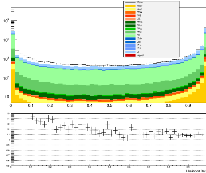
Figure 5.5: Distribution of likelihood ratio in lowest E_T^{\text{miss}} bin.
