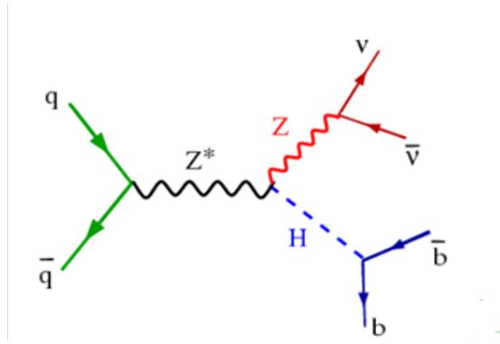
Figure 5.1: Feynman diagram for Higgs production in Higgs-strahlung production channel. The Z boson decays to neutrinos and H decays to a pair of b -quarks.
