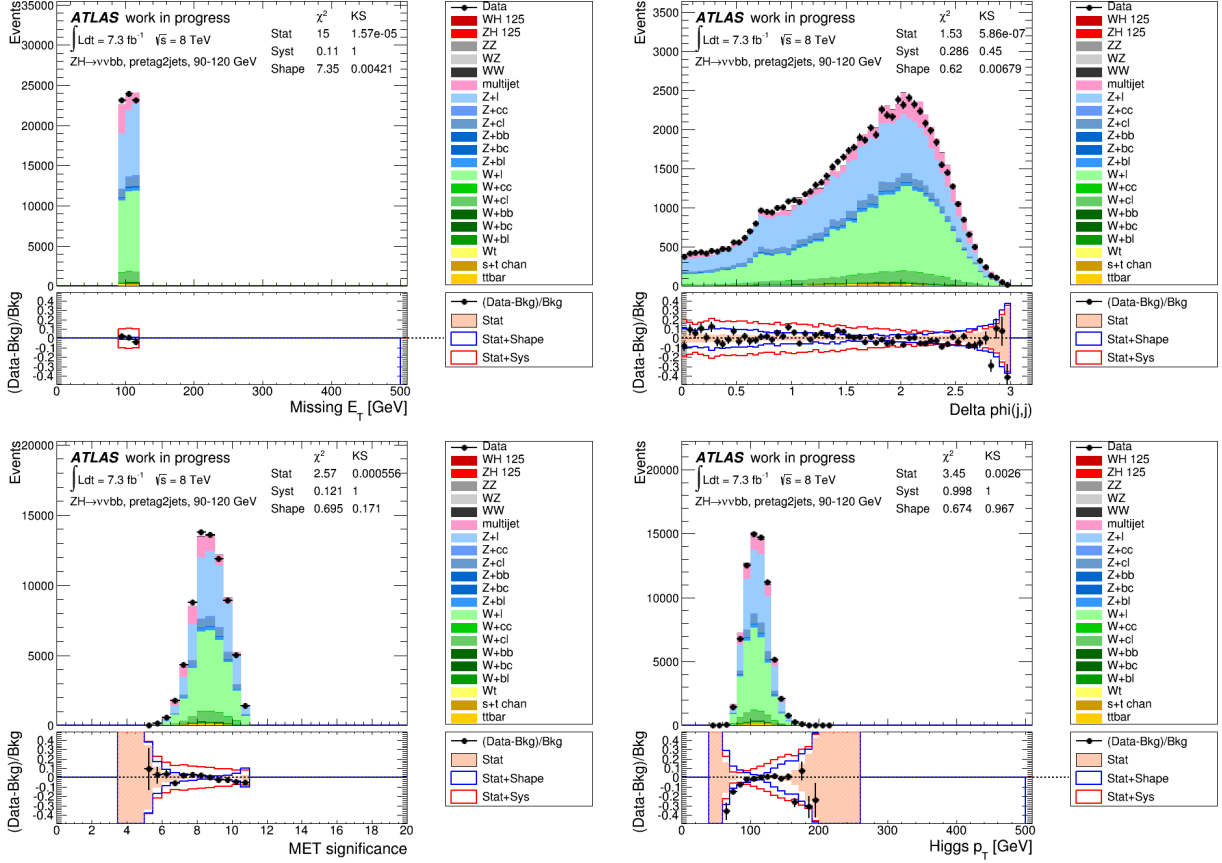
Figure 5.11: Distributions of event selection using delayed stream exclusively in first E_T^{\text{miss}} bin for E_T^{\text{miss}} (top left), \Delta\Phi(j, j) (top right), E_T^{\text{miss}} significance (bottom left), Higgs p_T (bottom right).
