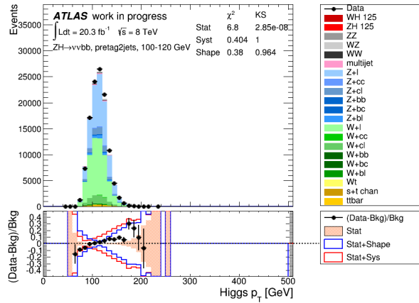
Figure 5.15: Distribution of Higgs p_T using nominal triggers with 100 < E_T^{\text{miss}} < 120 GeV.
