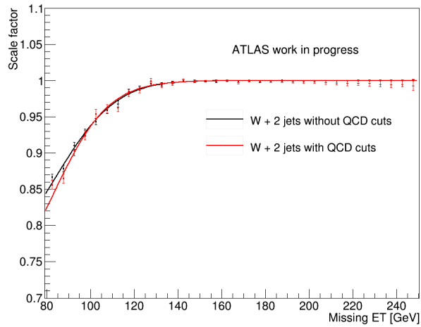
Figure 4.15: Comparison of total E_T^{\text{miss}} trigger turn-on from the fit curves of W \rightarrow \mu\nu between applying/not applying multijet rejection on MC (top) and data (middle) and trigger scale factor (bottom).
