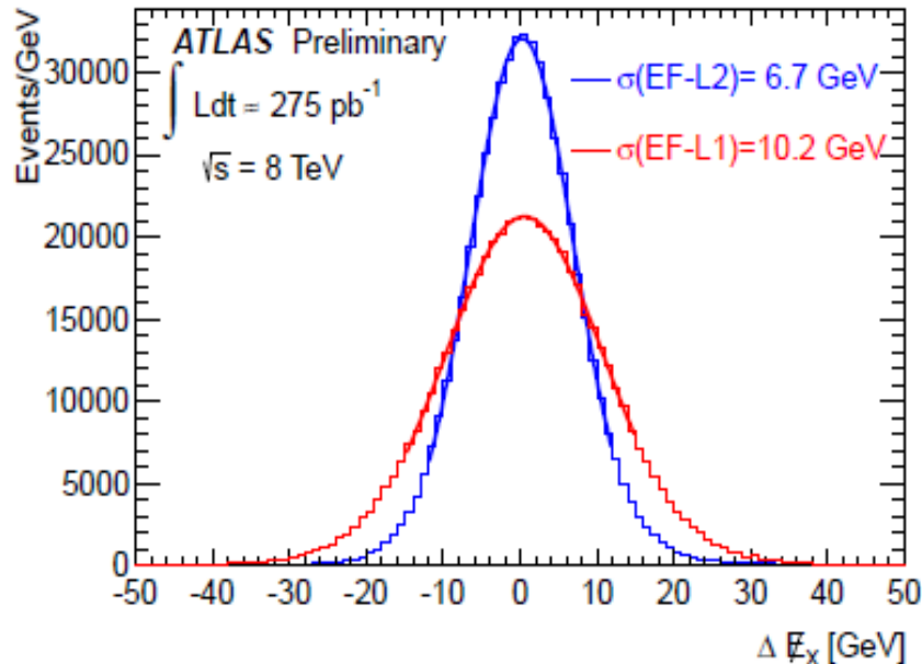
Figure 4.1: Resolution x -component of E_T^{\text{miss}} at L1 (red) and L2 (blue), which are measured with respect to EF of E_T^{\text{miss}} .
