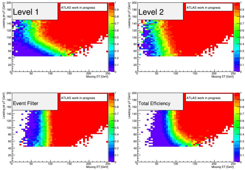
Figure 4.22: E_T^{\text{miss}} trigger turn-on dependence with respect to p_T of leading jet for trigger EF_xe80_tclw_loose for Z \rightarrow \mu\mu sample in 2-jet bin on MC. The colors correspond to the efficiency.
