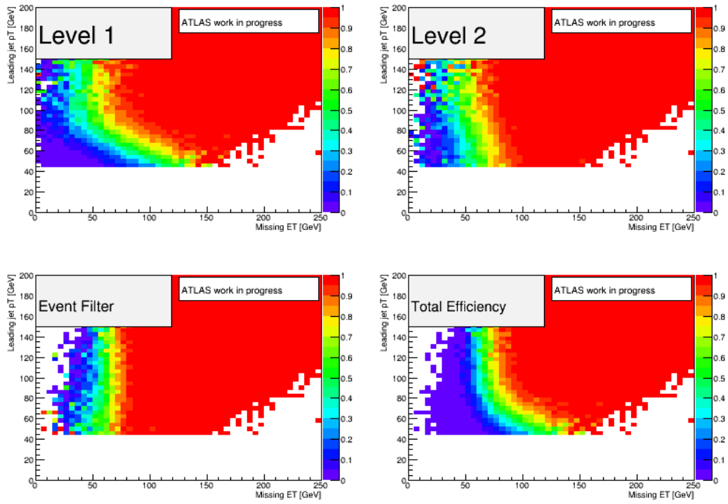
Figure 4.23: E_T^{\text{miss}} trigger turn-on dependence with respect to p_T of leading jet for trigger EF_xe60_tclw_loose_delayed for Z \rightarrow \mu\mu sample in 2-jet bin on MC. The colors correspond to the efficiency.
