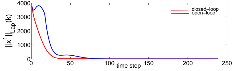
Figure 5.20: Evolution of the balancing metric for the link 1. The closed-loop system evidently improves the convergence rate.
