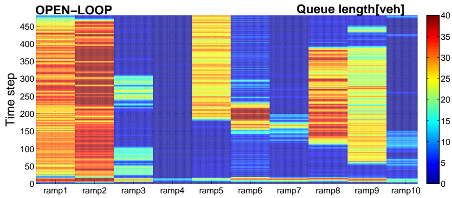
Figure 7.14: On-ramp queue lengths over time in the open-loop case.
