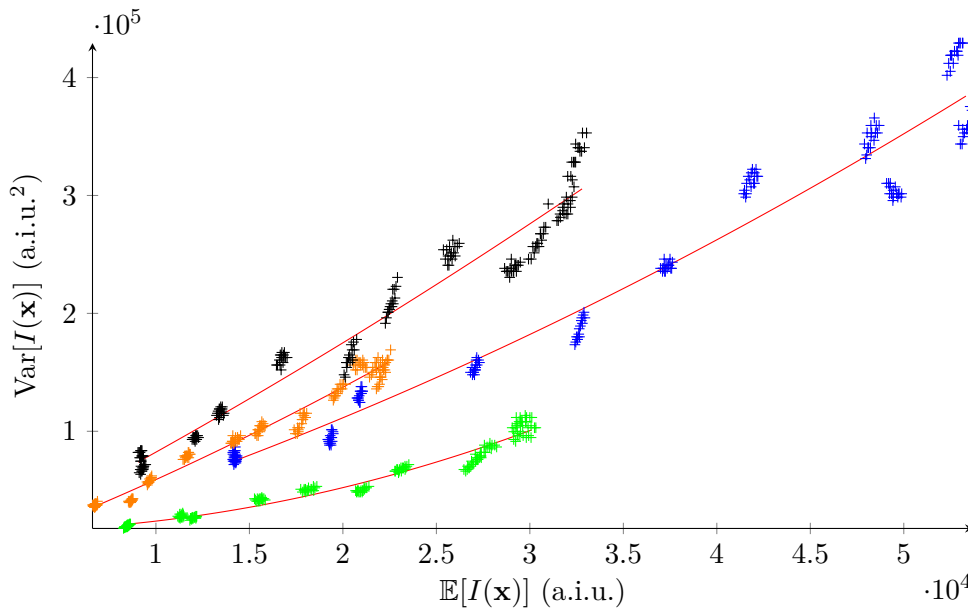
Figure 4.5: Four different gains at four different locations computed from a FD FLIM reference stack of 13 frames acquired with a confocal setup (crosses represent measured variances, lines represent the theoretical noise model).
