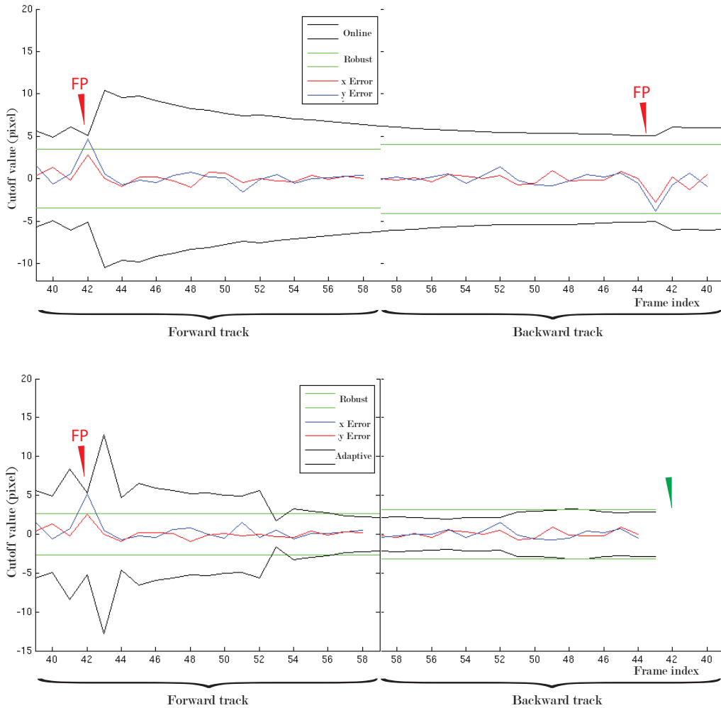
Figure 10.4: Impact of noise adaptation on linking cut-off for a single track. In this example, the low number of data points on the first few frames results in a weak estimate of the search radius leading to a false positive. Above, the process noise is computed using the iterative online estimator [Stengel, 1986]. As the method is not locally adaptive, it exploits all the prediction errors (Red and Blue lines) and repeats the tracking errors during backward tracking. Below, the process noise is computed using our method. By finally estimating the Kalman Filter process noise, we provide an accurate end of track time point on the backward tracking. The subsequent forward tracking does not repeat the previous mistakes (data not shown).
