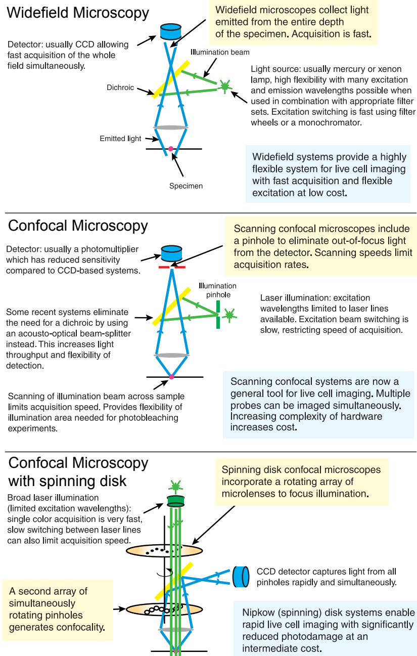
Figure 1.6: Comparison of wide-field, scanning confocal and spinning disk confocal systems, with schematics for each. All systems are capable of being equipped for 3D and 4D data acquisition. Excitation beams are shown in green; emission beams, in blue. The differences between these systems mean that no single system is suited for every experiment. Typical system configurations are shown, and user modification and options allow great flexibility (source: from [Stephens and Allan, 2003]).
