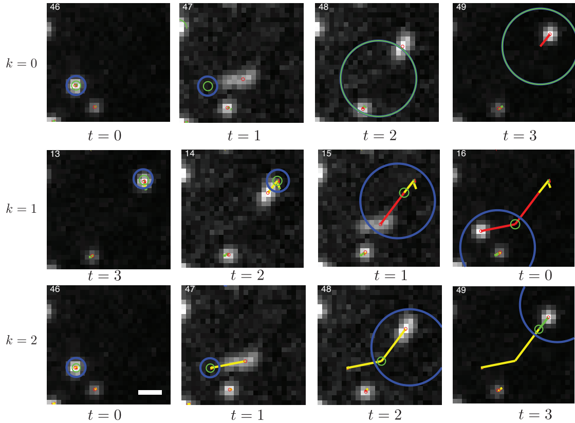
Figure 10.1: Convergence of speed estimation at the time point scale. Red links represent directed prediction selection, Green links represent Brownian prediction and Yellow represent prediction stemming from the previous tracking round. A small tracklet motion is easily retrieved during the first tracking round; it serves as a track initialization for the following track rounds (scale bar is 0.5 \mu m , acquisition frequency is 1Hz).
