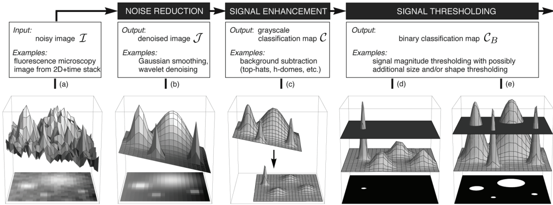
Figure 9.3: Object detection framework including noise reduction, signal enhancement and thresholding (source from: [Smal et al., 2010]).
