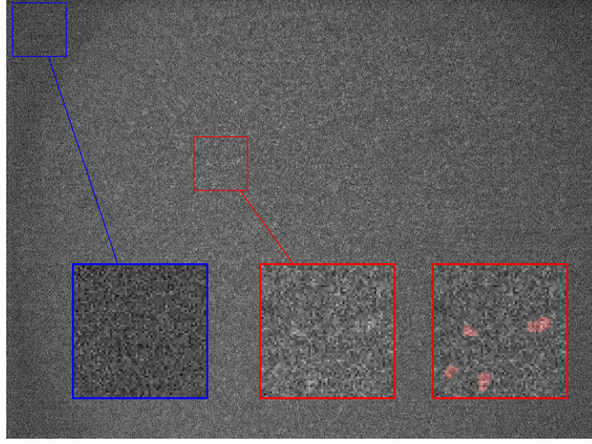
Figure 4.2: Spatial non-stationarity induced by the ICCD on a background image (an acquisition in the absence of excitation on ICCD input). Spontaneous burst of photon in the intensified area highlights the sensitivity of the device (raw intensity is presented on the middle magnification and automatically highlighted in red in the right magnification)). The blue-squared area is not intensified and describe a much more stationary intensity footprint for the CCD.
