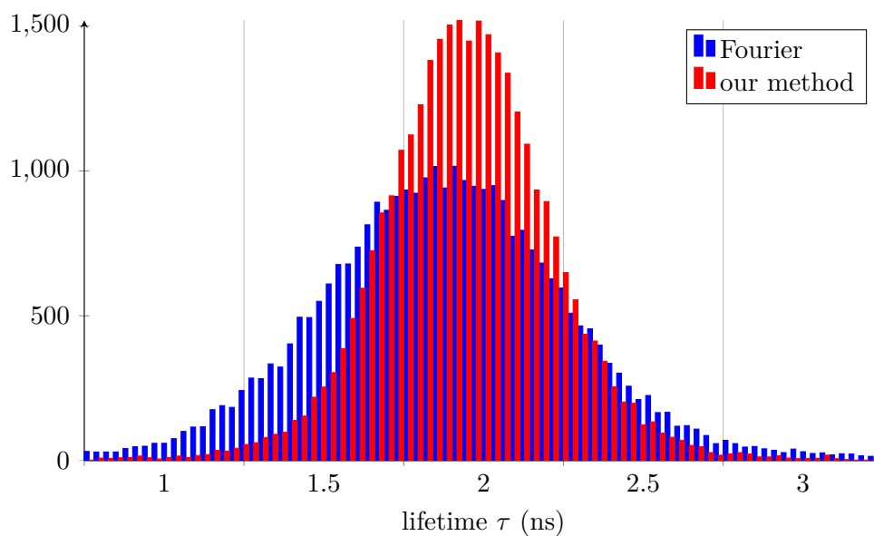
Figure 4.10: Lifetime histograms on the whole image control cells with GFP tagged receptor in live cell RPE1.
