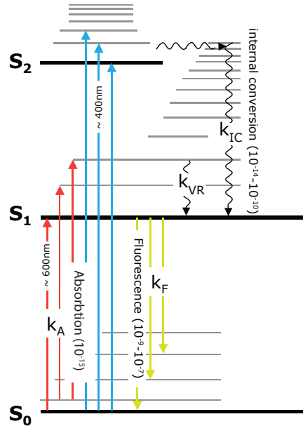
Figure 1.1: Simplified Jablonsky diagram. The thick horizontal lines denote electronic energy levels. The thinner grey lines represents the various vibrational energy states. Straight arrows are associated with absorption or emission of a photon. Wavy arrows illustrate molecular internal conversions or non-radiative relaxation processes. Vertical upward arrows indicate the instantaneous nature of excitation processes.
