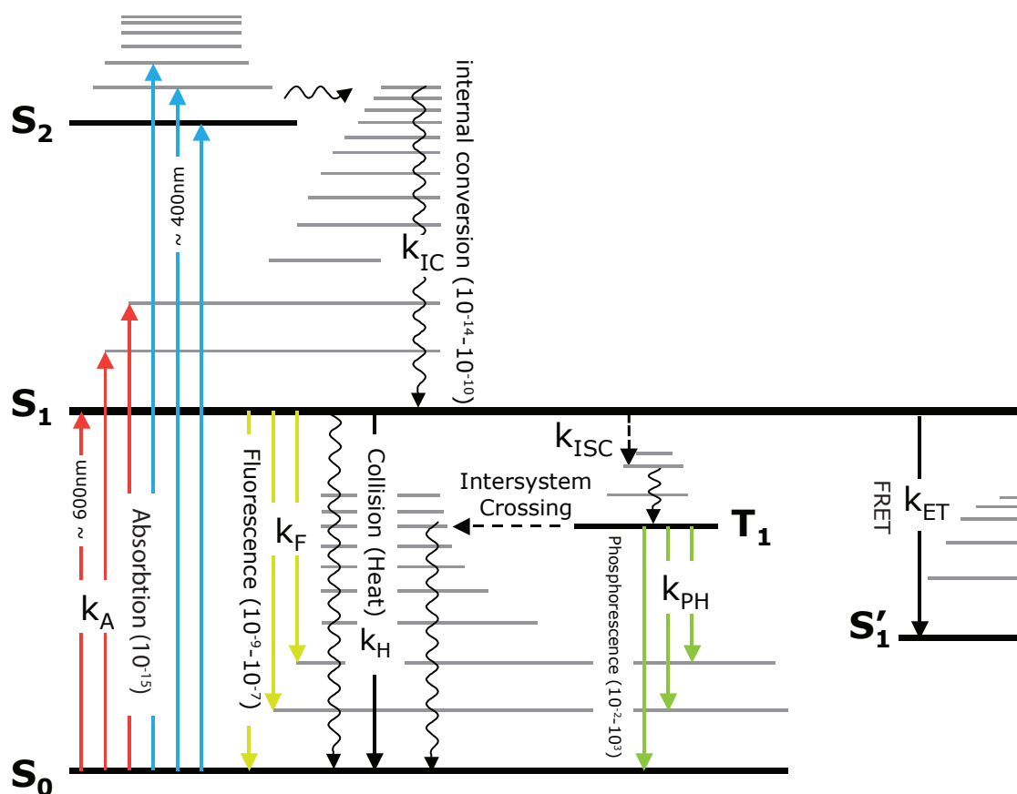
Figure 2.1: Jablonsky diagram: the thicker lines represent electronic energy levels and the thinner lines denote the various vibrational energy states. A timescale for the transition or a color is given as an example when physically meaningful.
