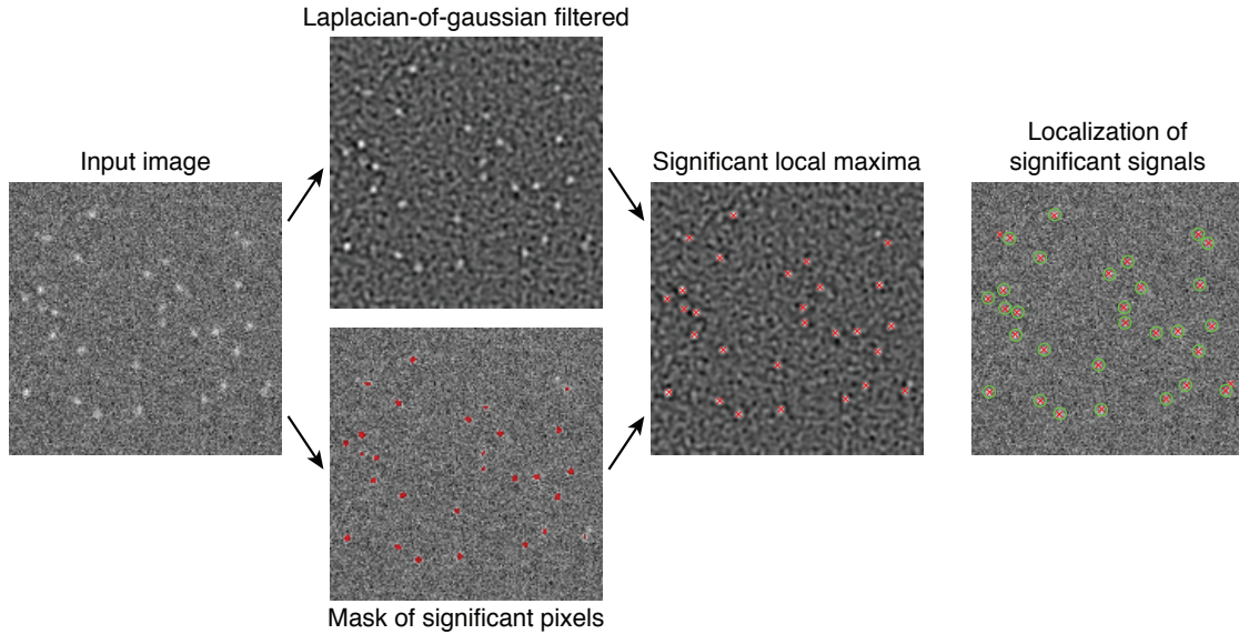
Figure C.2: Detection workflow as described in [Aguet et al., 2013].
