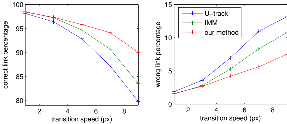
Figure 10.8: Correct linking and false positive percentage wrt transition speed.
