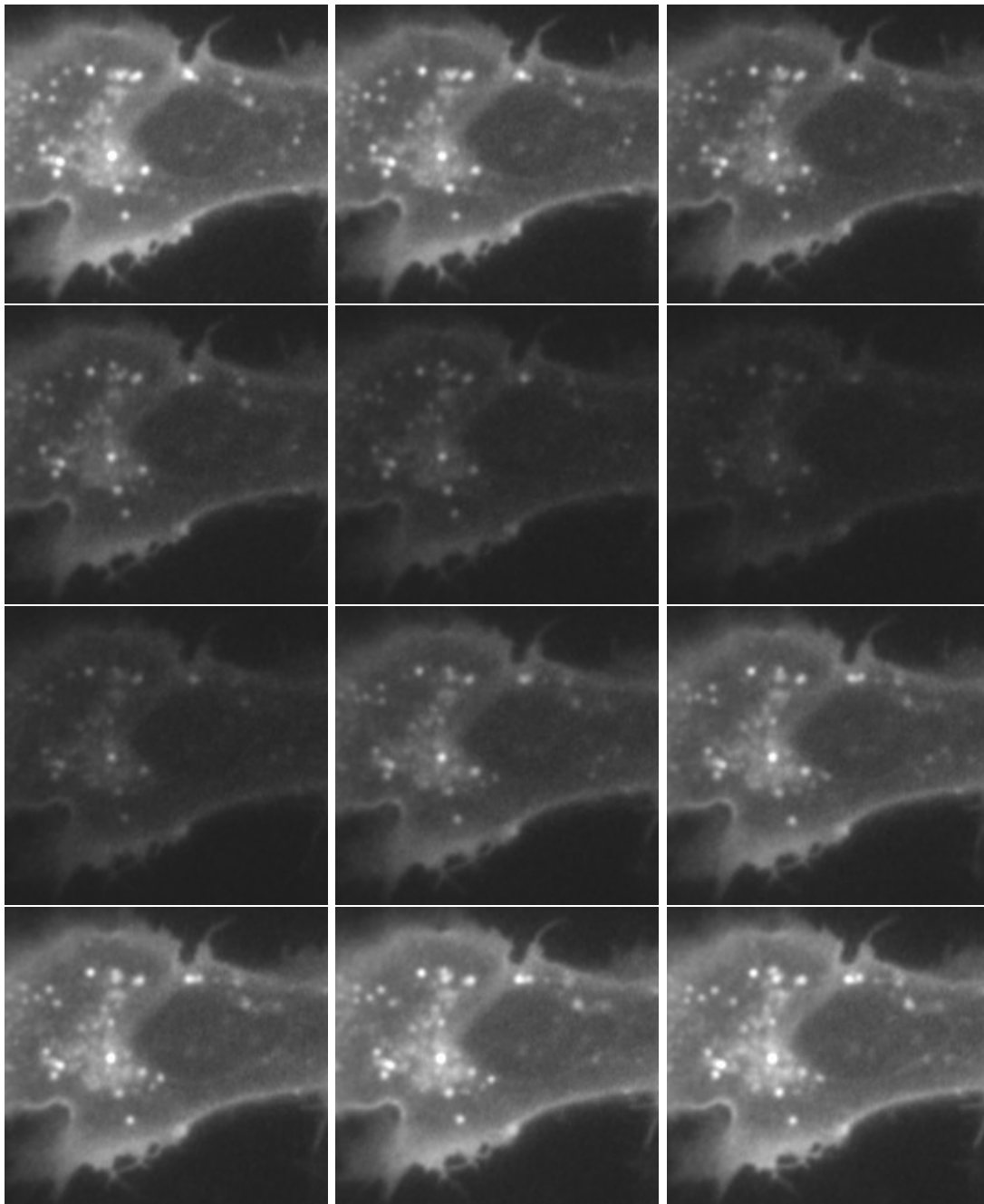
Figure 3.4: An example of FD FLIM measurement with K = 12 phase-modulation signals. The sequence must read from the upper left to the lower right. Fluorescent structures localize receptors tagged with GFP in epithelial cells (RPE1). Contrast has been artificially enhanced on the image presenting low intensity for visualization purpose.
