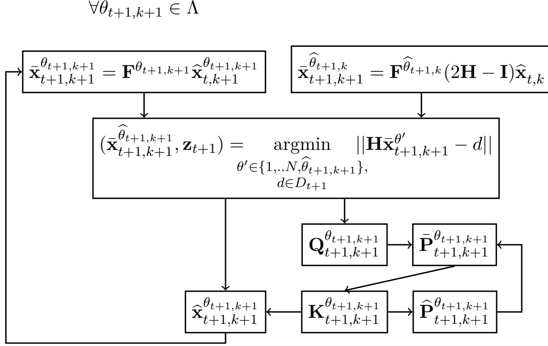
Figure 10.2: Overview of our tracking algorithm at tracking round k+1 . Let D_{t+1} be the detection (measurement) set at time t+1 . For each measurement, the closest prediction \bar{\mathbf{x}}_{t+1,k+1}^{\hat{\theta}_{t+1,k+1}} is selected by the among predictions made by N Kalman filters at round k+1 and the estimated posterior at round k . The graph-based combinatorial algorithm [Jonker and Volgenant, 1987] estimates the optimal assignment (\bar{\mathbf{x}}_{t+1,k+1}^{\hat{\theta}_{t+1,k+1}}, \mathbf{z}_{t+1}) between the closest prediction and detections for every track. Once the best measurement is assigned to the track, this measurement is used to update each Kalman filter variable independently.
