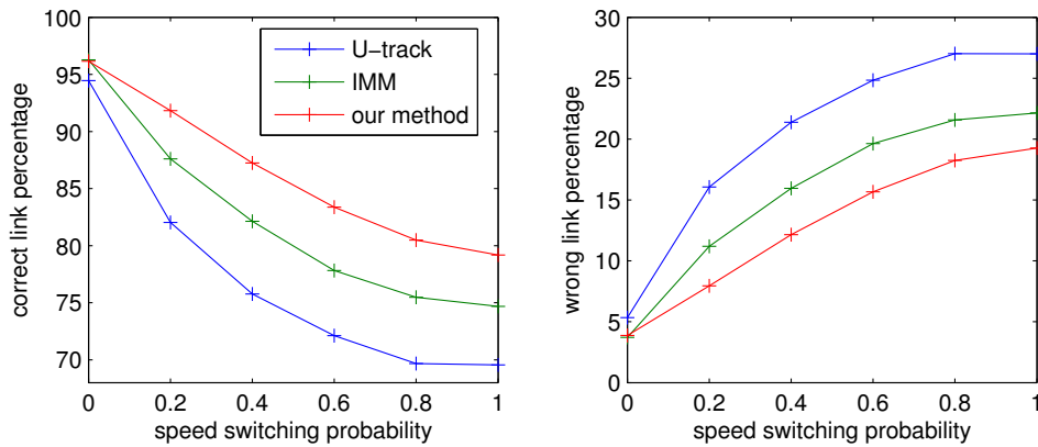
Figure 10.9: Correct linking and false positive percentage wrt speed switching probability.
