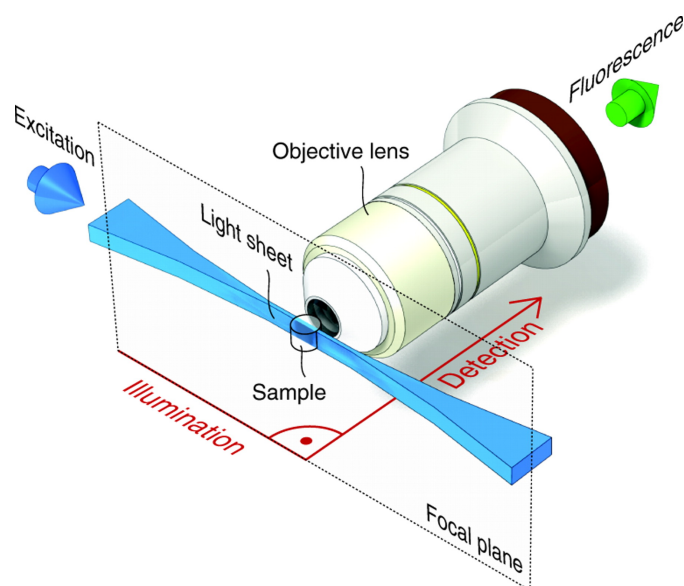
Figure 1.8: Schematic representation of SPIM principle (source: from a scheme by Jan Krieger)
