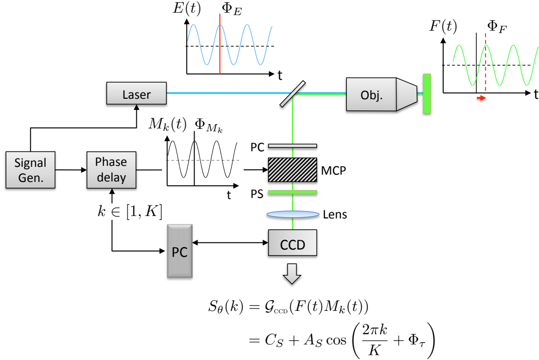
Figure 3.3: Instrumental setup showing the different elements of the system and the corresponding signals for FD FLIM. E(t) denotes the excitation light, F(t) the fluorescence signal, M_k(t) the detection modulation signal and S_{\theta} is the resulting FD FLIM measurement.
