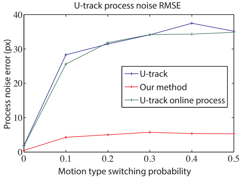
Figure 10.7: Process noise estimation error on simulation wrt motion switching probability: 0 means pure Brownian motion, 0.5 means a rate of 50% chances to switch to direct or Brownian motion. Vesicle density is set to 3 spots/ \mu\text{m}^2 . Our method is compared with process-noise variance estimation on the whole track up to time t (u-track) and an online and iterative though non adaptive process noise variance estimation (u-track online process).
