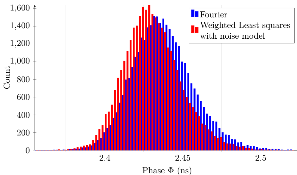
Figure 4.9: Phase histograms using the Fourier method and the weighted least squares method exploiting the estimated noise scale on a reference FD FLIM measurement of a plain fluorescein sample (see Figure 4.3.a).
