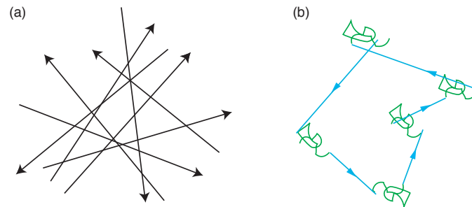
Figure 8.4: Heterogeneous motion model on a disordered cytoskeleton network (a) and associated vesicle trajectory undergoing switches between confined diffusion and directed motion (see [Bressloff and Newby, 2013]).
