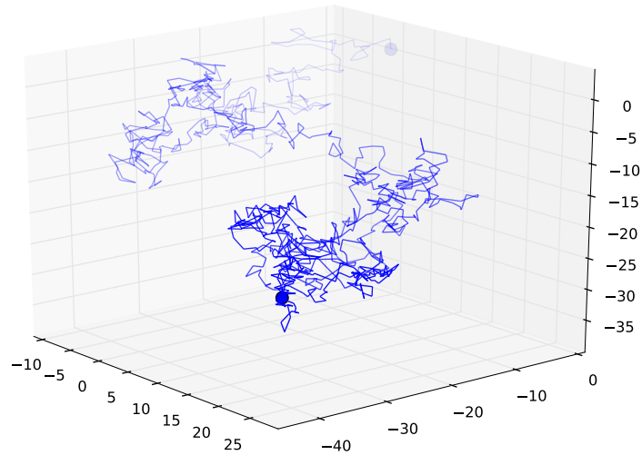
Figure 8.1: Trajectory of a single molecule undergoing Brownian motion in three dimensions. Segment color strength indicates temporal progression.
