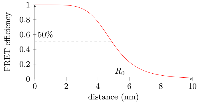
Figure 2.2: FRET efficiency evolution with the distance r between fluorophores ECFP and EYFP ( R_0=4.9 nm).
