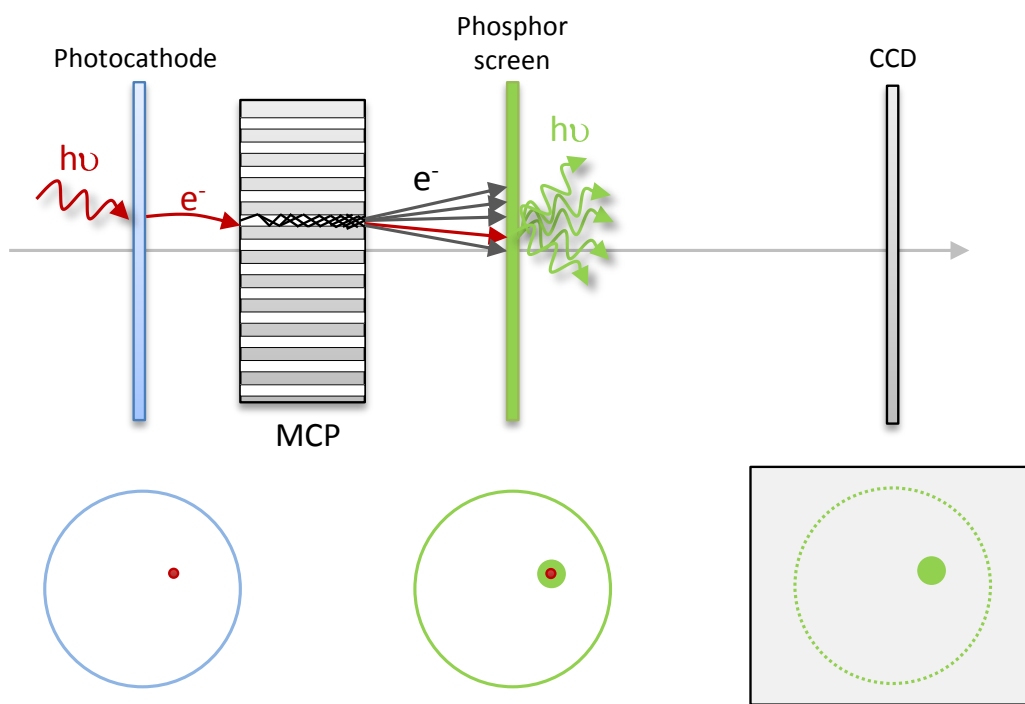
Figure 4.1: Image formation process in a third generation Intensified CCD.
