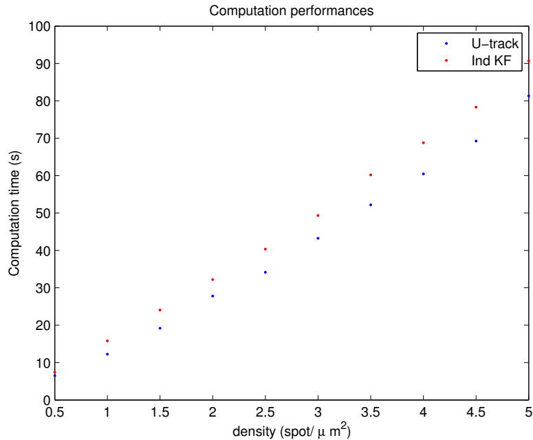
Figure 10.11: Computation time measured on the tracking alone (no detection). Mixture of confined diffusion (50%), free diffusion (40 %) and direct motions (10%). Computation overhead is around 10% with respect to u-track. The complexity grows linearly with density.
