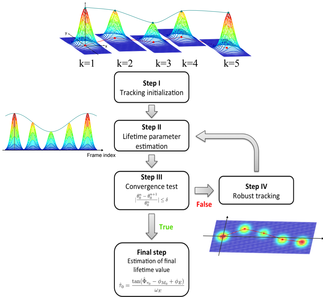
Figure 5.4: Iterative and alternative procedure for fluorescence lifetime estimation on moving endosomes.
