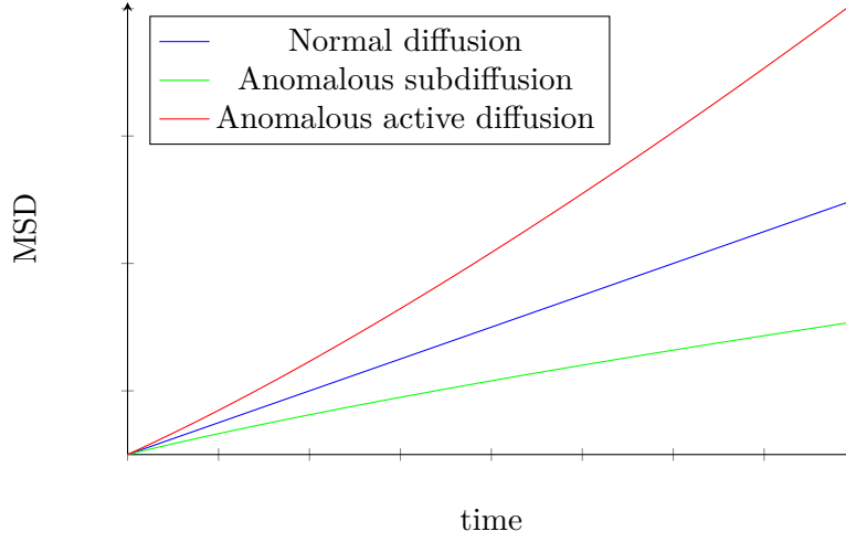
Figure 8.3: Simulation of anomalous subdiffusion and active diffusion as a function of time.
