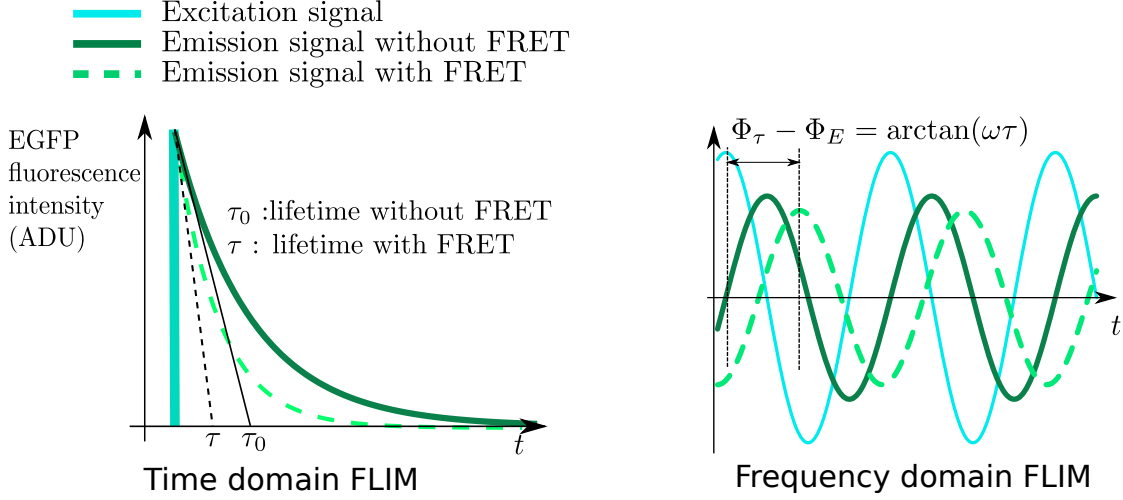
Figure 3.1: Representation of lifetime measurement and effect of a fluorescence lifetime loss in the time domain and frequency domain.
