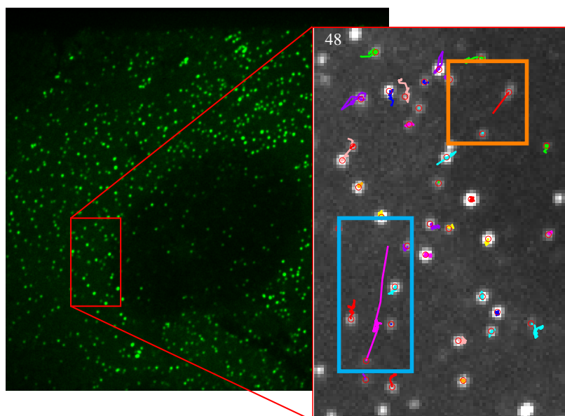
Figure 8.7: Vimentin motility seems to present a large proportion of confined Brownian motion and rare, sudden, motor-mediated transport. Vimentin null epithelial cell (cell line SW13) transfected with ULF of vimentin Y117L mutant fused to GFP. Image acquired with a spinning disk confocal microscope with a 100x objective zoom 1.5 (Numerical Aperture 1.4, pixel size 0.10905 \mu\text{m}/\text{pixel} ). Colored Tracks have been computed with an advanced u-track parametrization. This quantification is not perfect as demonstrated in Figure 8.8. However, u-track manages to highlight a large directed motion in a dense population of Brownian moving particles.
