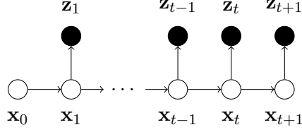
Figure 9.4: Dependency graph of a Hidden Markov process applied to the state \mathbf{x}_t and measure \mathbf{z}_t , \forall t \in \mathbb{N} .
