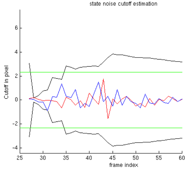
(a) U-track needs a few frames to calibrate the noise process.
