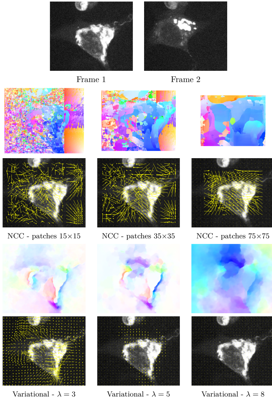
Figure 13.6: Results on the “HeLa cell” sequence (acquisition by Perez’ group, UMR 144 Institut Curie, PICT-IBiSA). 1^{st} row: two input images. 2^{nd} and 3^{rd} rows: color and arrow visualizations of the results obtained with the NCC block matching, for several patch sizes. 4^{th} and 5^{th} rows: color and arrow visualizations of the results obtained with the variational method, for several regularization coefficients.
