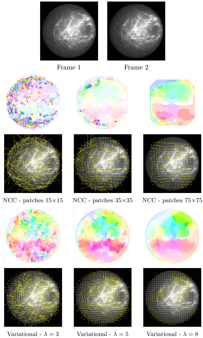
Figure 13.5: Results on the “Actin network” sequence Pinot et al. [2012]. 1 st row: two input images. 2 nd and 3 rd rows: color and arrow visualizations of the results obtained with the NCC block matching, for several patch sizes. 4 th and 5 th rows: color and arrow visualizations of the results obtained with the variational method, for several regularization coefficients.
