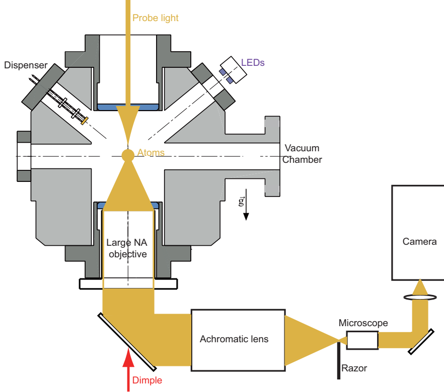
Figure 2.13: The optical imaging system of the absorption imaging
