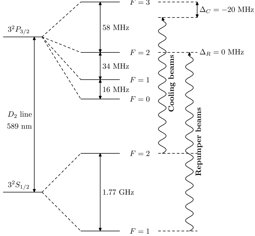
Figure A.2: Sodium energy structure with cooling and re-pumping lasers, with respective detunings \Delta_c and \Delta_R with respect to the 2 \rightarrow 3 and 1 \rightarrow 2 transitions.
