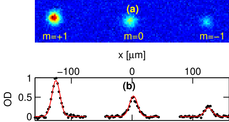
Figure 3.1: (Color online) a: Absorption image of a spin 1 BEC after expansion in a magnetic gradient. b: Horizontal cuts through the images in (a). The same function (shown by straight lines), only recentered and reweighted, is used to fit the density profile of each Zeeman state.
