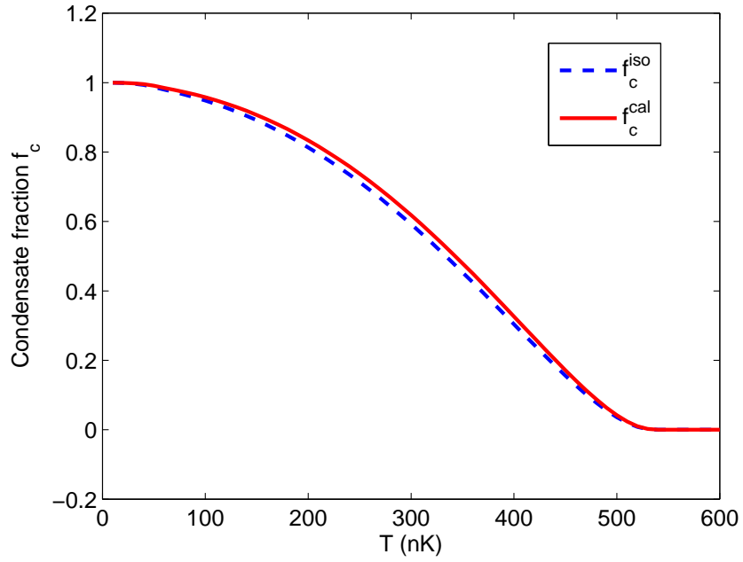
Figure 1.9: Comparison between f_c^{\text{cal}} and f_c^{\text{iso}} at q = 0 .
