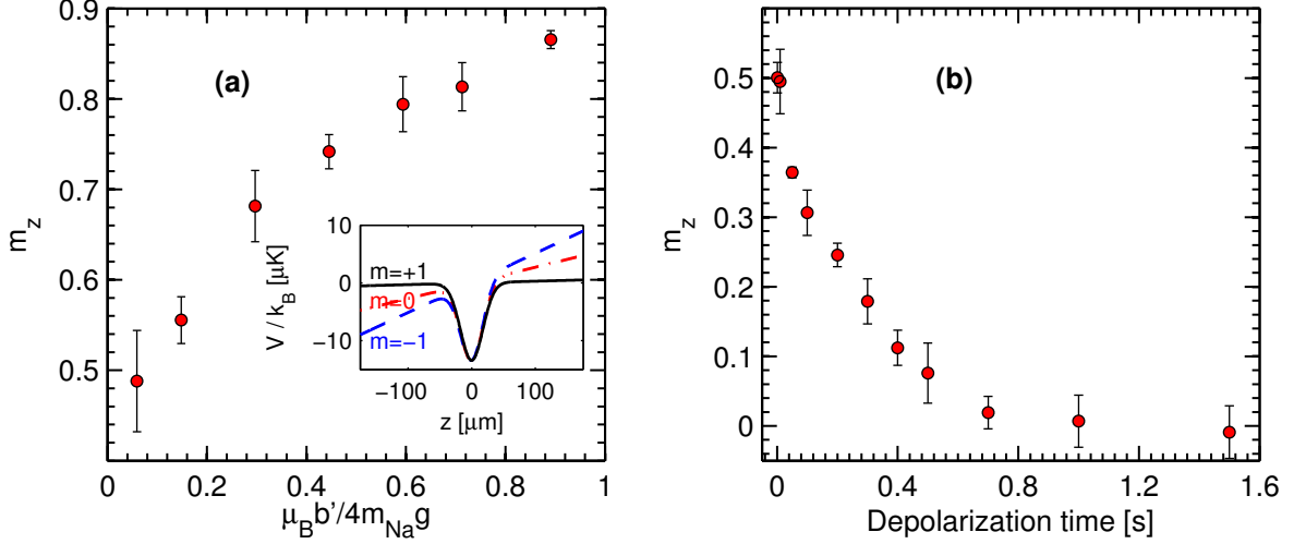
Figure C.1: Supplementary Material- (Color online) (a): Spin distillation to prepare samples with high magnetization ( m_z > 0.5 ). The plot shows the magnetization measured for cold clouds, as a function of the magnetic gradient b' in units of m_{\text{Na}}g/\mu_B , with g the acceleration of gravity and \mu_B the Bohr magneton. The inset shows a sketch of the potential energies for each Zeeman state along the vertical axis z . The potential drop is exaggerated for clarity, and is smaller than depicted in the actual experiment. (b): Depolarization to prepare samples with low magnetizations ( m_z < 0.5 ). The time shown corresponds to the length of a radio-frequency pulse at the Larmor frequency.
