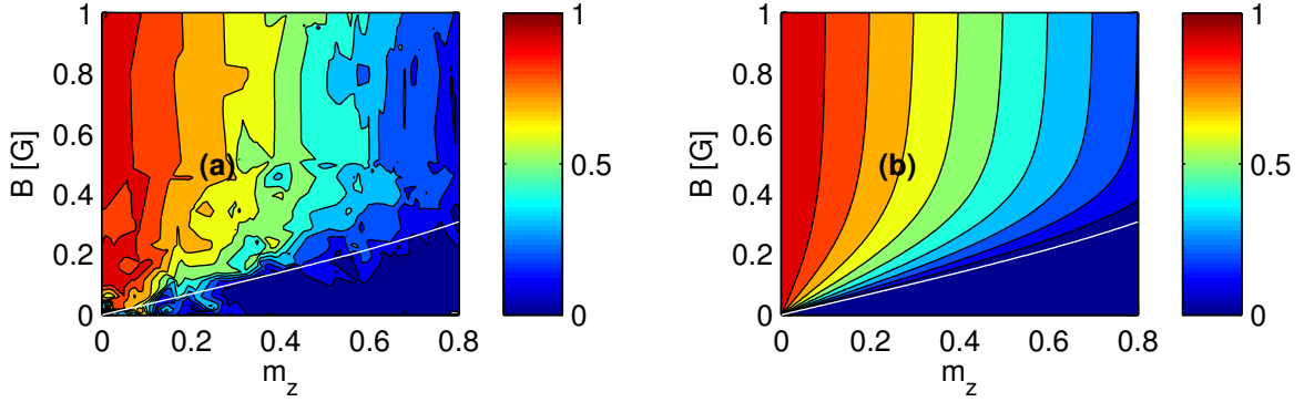
Figure 3.3: (Color online) a: Experimental phase diagram showing the population n_0 of the m = 0 Zeeman state versus magnetization m_z and applied magnetic field B . The plot shows a contour interpolation through all data points, with magnetization ranging from 0 to 0.8. The white line is the predicted critical field B_c separating the two phases, deduced from Eq. (3.4) by q_c = q_B B_c^2 . b: Theoretical prediction for n_0 at T = 0 K.
