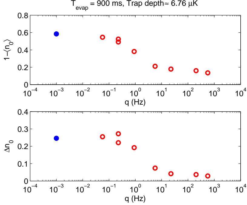
Figure 4.1: Second evaporation T_{\text{evap}} = 900 ms, trap depth \sim 6.76 \mu\text{K} , hold time 6 s. The point closet to q = 0 (the solid blue circle) corresponds to zero applied field, and has been set arbitrarily at q = 10^{-3} Hz.
