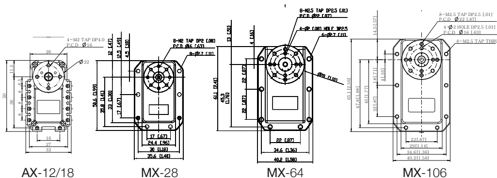
Fig. 5.5.: The footprint of Dynamixel motors keeps the same pattern, only the dimensions are increased following the power of the motor. Thus, switching from one model to another only requires changing the dimension and not the design of a part. With parametric CAD software such as Solidworks, it takes a couple of minutes to modify a mechanical part to be compatible with another Dynamixel motor.
