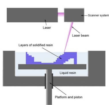
(a) SLA process
