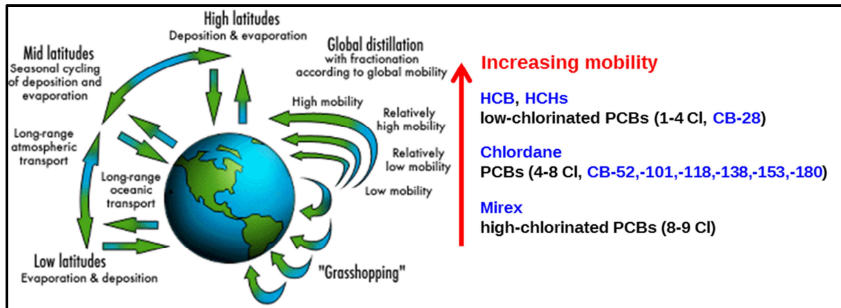
Fig. 2. Schematic representation of POPs migration processes (modified from Wania and Mackay 1996 ). Some of the pesticides and PCBs studied during the doctoral work are presented in blue, sorted in increasing mobility.
