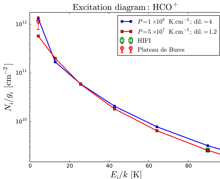
Figure 107: Observable excitation diagram of HCO + for the best model (blue, P = 1 \times 10^8 \text{ K.cm}^{-3} , A_V = 5 ), compared to a lower pressure model, and to our observational constraints.
