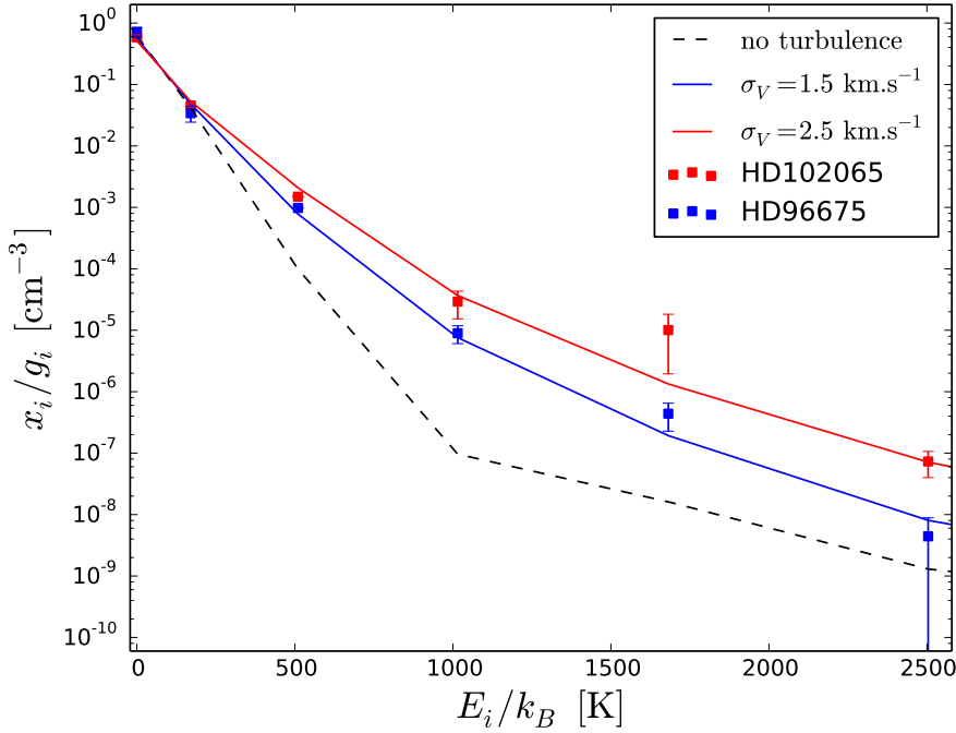
Figure 95: Models with n_H = 40 \text{ cm}^{-3} fitting two specific lines of sights from Gry et al. [2002].
