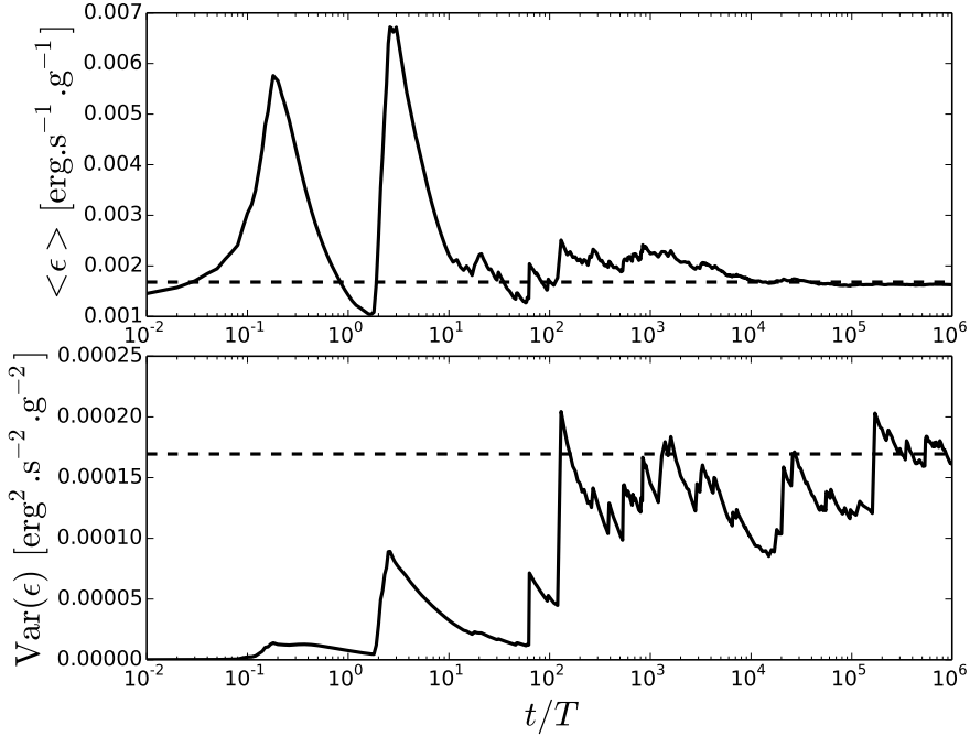
Figure 80: Convergence of the mean and the variance of the dissipation rate \epsilon in a simulation. The dashed lines show the theoretical values.
