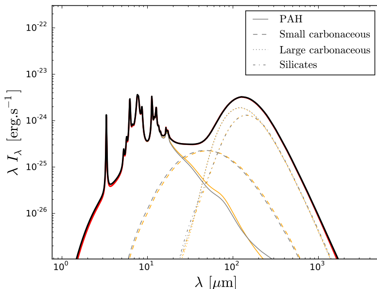
Figure 44: Emission spectra of dust, comparing our computation (black and grey lines) to the DustEM code (red and orange lines). The thin lines represents the emission of the different dust components, while the thick lines show the total emission. The emission is given per hydrogen gas atom, for a dust population following the DustEM dust model (Compiègne et al. 2011, see Sect. 5.3.3) irradiated by an external radiation field with \chi = 1 .
