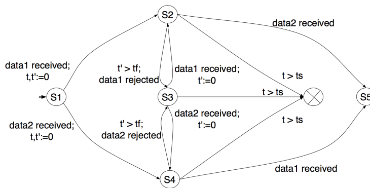
FIGURE 6: Automate de temporisation
