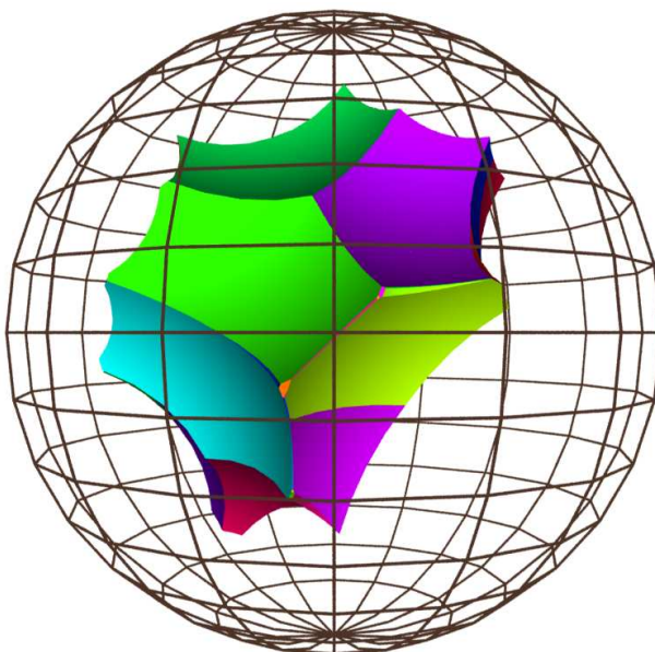
FIGURE 5. Dirichlet domain of \mathbb{H}\left(\mathbb{Z}\left[\frac{1+\sqrt{-7}}{2}\right]\right)^1
