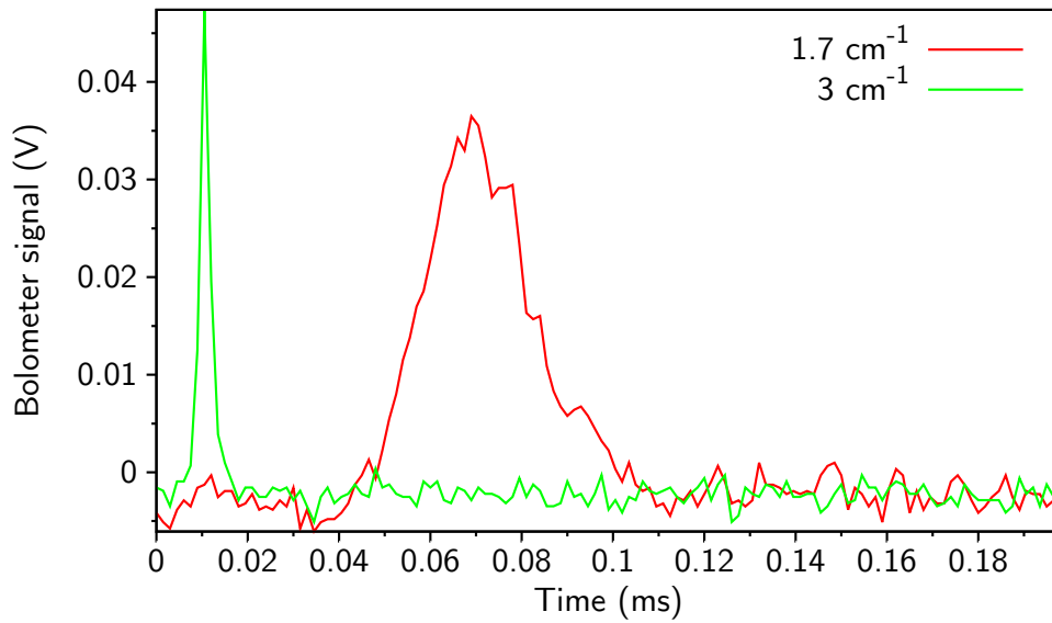
FIGURE 4.7: Bolometer signal versus time for two excitation wavenumbers: 1.7 \text{cm}^{-1} (red) with a strong delayed response, signature of the seeding effect, and 3 \text{cm}^{-1} (green) with no delayed response. The beam current is I = 7 mA.
