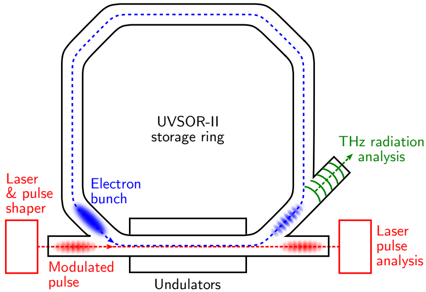
FIGURE 4.1: Experimental setup on the UVSOR-II storage ring. An electron bunch interacts with a modulated laser pulse in an undulator. Then, the electrons emit coherent terahertz radiation over several turns.
