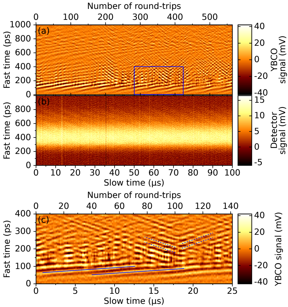
FIGURE 5.6: (a,c) Color map of the temporal evolution of the CSR electric field above the instability threshold ( I = 62 mA). (c) Zoom of (a) between 50 and 75 \mu s (blue box in (a)). (b) Associated temporal evolution of the longitudinal electron bunch profile measured with the EOT photodetector.
