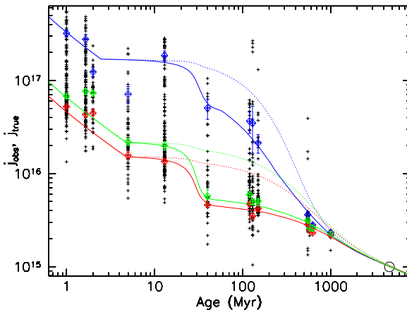
Fig. 6. Observed specific angular momentum ( j_{obs} = I_* \Omega_{env}/M_* ) evolution (solid line) and actual specific angular momentum ( j_{true} = (I_{core} \Omega_{core} + I_{env} \Omega_{env})/M_* ) evolution (dotted line) for the fast (blue), median (green), and slow (red) rotator models. The blue, green, and red tilted squares represent respectively the 90 th , 50 th , and 25 th percentiles of the observed specific angular momentum computed from the cluster's rotational distributions. The open circle is the specific angular momentum of the present-day Sun.
