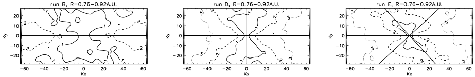
FIG. 8.—Runs B, D and E. Visualizing the radial energy damping rate in Fourier space. Lines: isocontours of radial damping rate of total energy spectra in the (K_x, K_y, K_z = 0) plane. The radial damping rate \alpha is given by E(t_1)/E(t_0) = (R(t_1)/R(t_0))^{-\alpha} , with t_0 = 1.4, t_1 = 1.8 and R(t_0) = 0.76, R(t_1) = 0.92 . (represented with vertical dotted lines in fig. 9). Left panel, run B (no mean magnetic field); middle panel, run D (radial mean magnetic field); right panel, run E (oblique mean magnetic field). Thin lines indicate the directions parallel and perpendicular to the mean magnetic field when present.
