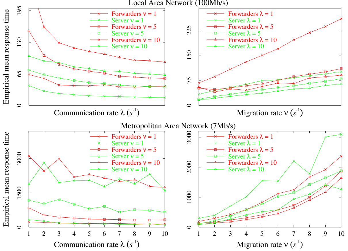
Figure 3.10: Experimental results obtained on a LAN and a MAN
