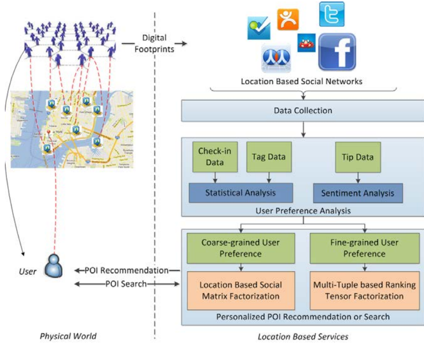
Figure 4.1: Sentiment-enhanced personalized POI recommendation and search framework.
