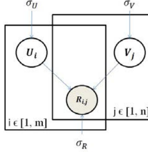
Figure 4.6: Graphical model of probabilistic matrix factorization.
