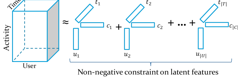
Figure 5.5 – Non-negative tensor factorization using Canonical decomposition model.
