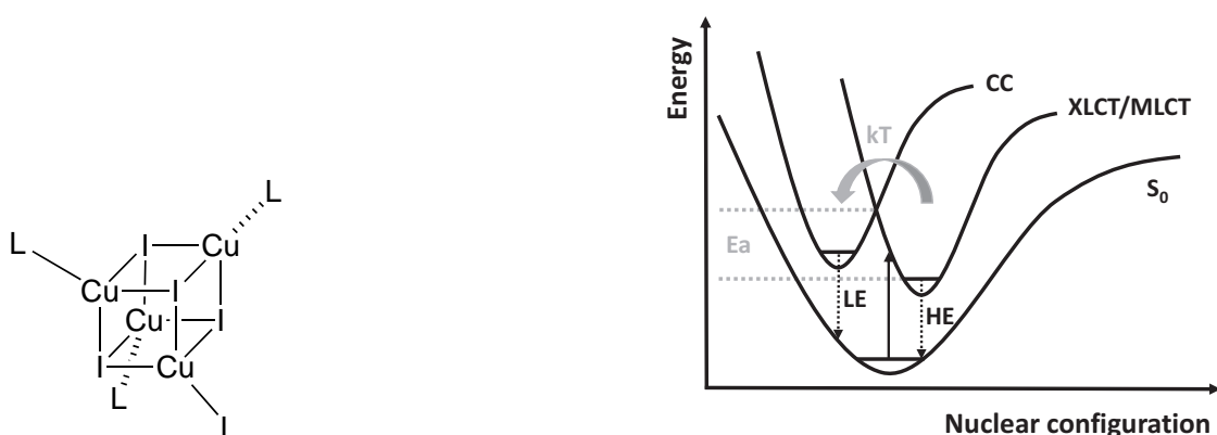
Figure 2.4: Left: General representation of [\text{Cu}_4\text{I}_4\text{L}_4] -clusters ( X = \text{Cl}, \text{Br}, \text{I} ; L = organic ligand). Right: Simplified energy level diagram of the copper iodide clusters studied.
