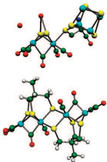
Figure 3. (top) Structure of \text{H}_{\text{ox}} as determined by X-ray crystallography of the oxidized form of the [Fe–Fe] hydrogenase from C. pasteurianum (PDB ID 1C4A). 2 Note in this published structure the atoms forming the dithiolate bridge were not refined nor assignment of the diatomic ligands as either CO or cyanide made (see Scheme 1). (bottom) DFT-calculated structure of \text{Fe}_4\text{S}_6^{2-} .
