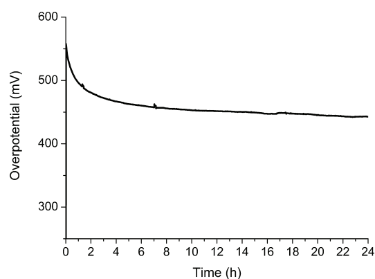
Figure 7. Galvanostatic control experiment on an electrode functionalized with FeS nanoparticles dispersed in Nafion (overpotential = | applied potential + 0.059 × pH| vs NHE). The experiment was performed on a rotating disk electrode in 0.1 mol/L potassium phosphate buffer at pH 7.0 and 20 °C ( I = 50 \mu\text{A} ; rotation rate 4000 rpm). No quantifiable pH variation during the experiment was observed.
