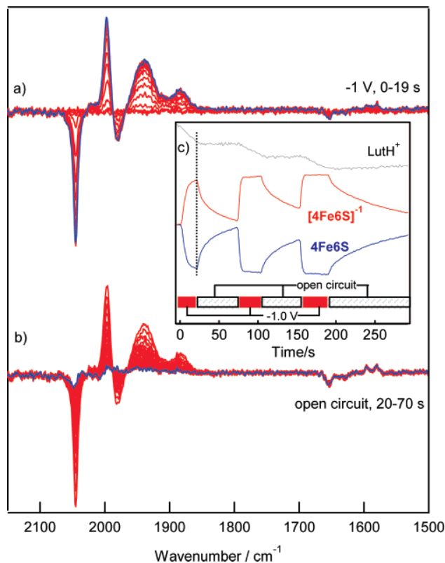
Figure 4. IR-SEC recorded of 4Fe6S (1.7 mM, CH 2 Cl 2 /0.2 M TBA[PF 6 ]) in the presence of LutH + (34 mM) (a) during the reduction at potentials sufficient to generate the monoanion, (b) the spectral changes obtained after switching the potentiostat to open circuit, and (c) the time dependence of the relative concentrations of LutH + , 4Fe6S , and 4Fe6S - obtained by multicomponent fitting of the individual spectra. The last spectrum of each set shown in a and b is highlighted.
