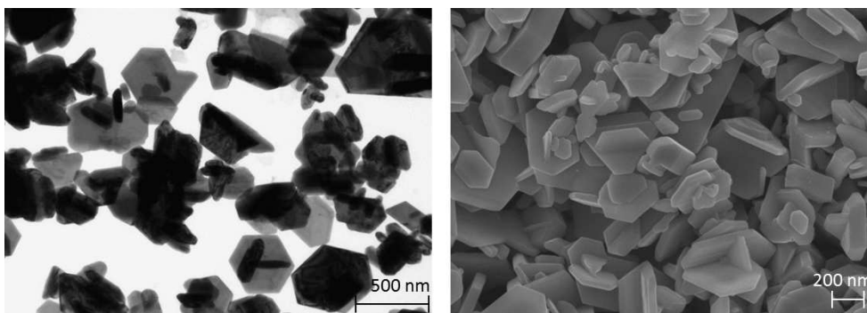
Figure 2.23: TEM and SEM images of FeS-nanoparticles.
