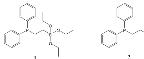
Figure 2. Phosphine ligands studied: 1 = \text{PPh}_2(\text{CH}_2)_2\text{Si}(\text{OCH}_2\text{CH}_3)_3 , 2 = \text{PPh}_2(\text{CH}_2)_2\text{CH}_3 .
