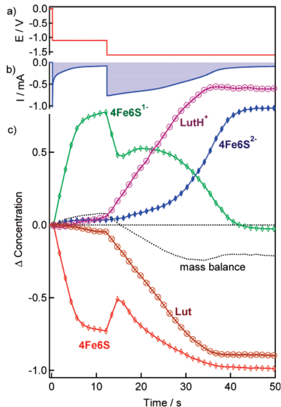
Figure 5. The time dependence of (a) the applied potential, (b) current response, and (c) the time dependence of the concentration changes of 4Fe6S , 4Fe6S - , 4Fe6S 2- , Lut, and LutH + during thin-layer SEC of 4Fe6S (1.1 mM) and LutH + (38 mM) in CH 2 Cl 2 (0.2 M TBA[PF 6 ]). The concentration changes of Lut and LutH + have been divided by a factor of 40. The mass balance of 4Fe6S - species corresponds to the sum of the concentration changes for 4Fe6S , 4Fe6S - , and 4Fe6S 2- .
