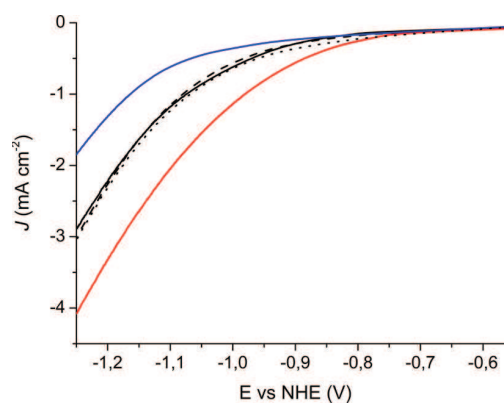
Figure 8. Linear sweep voltammetry of FeS nanoparticles dispersed in Nafion. Voltammograms were recorded on a rotating disk electrode in 0.1 mol/L potassium phosphate buffer at pH 6.0, 7.0, and 8.0 at 20 °C (scan rate 0.01 V/s; rotation rate 4000 rpm). Initial pH 7.0 conditions (solid black line); pH 6.0 (red line); pH 7.0 restored conditions from pH 6.0 (dashed line); pH 8.0 (blue line); pH 7.0 restored conditions from pH 8.0 (dotted line).
