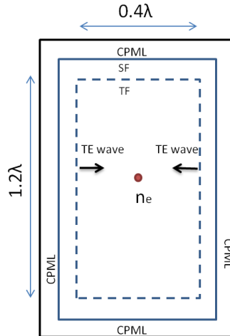
Figure 2.12: Simulation domain and dimensions.
