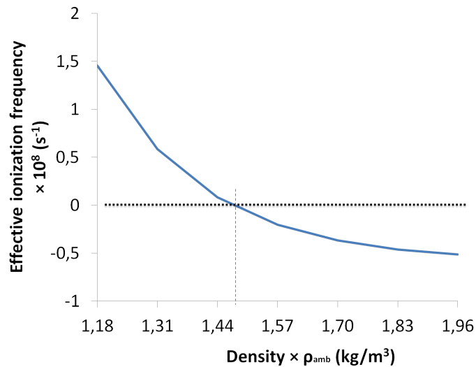
Figure 2.46: Effective ionization frequency versus gas density.
