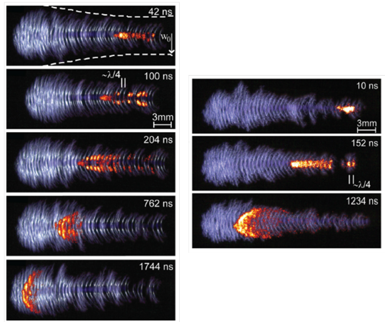
Figure 2.21: Open-shutter (background image, blue) and fast-gated (overlay, orange) photographs of break-downs with linearly (left) and circularly (right) polarized beam [63].
