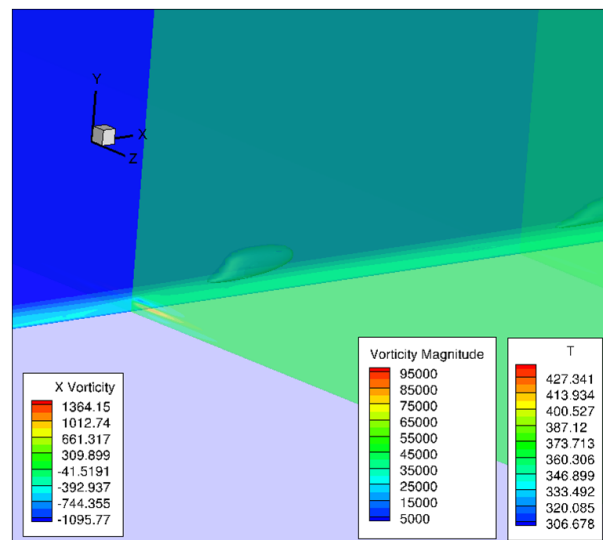
Figure 1.40: Temperature iso-surfaces, x -vorticity contours ( zy planes) and vorticity magnitude contours ( xy plane) at t = 4ms
