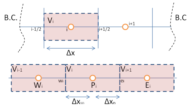
Figure 1.72: A central finite volume discretization of an one dimensional problem.
