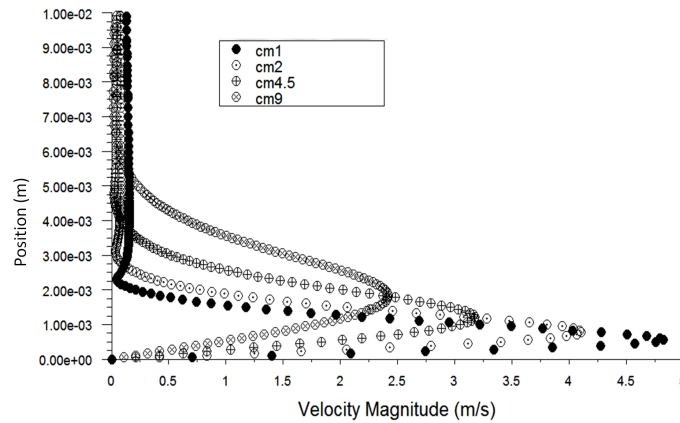
Figure 3.20: Velocity profiles at 1, 2, 4.5 and 9 cms from the plasma zone. Laminar assumption of the flow.
