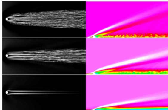
Figure 1.6: Transition provocation due to a hemispherical bump over a flat plate at M=3.3, 5.2, 8.2 (from up to down)[5].
