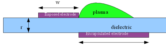
Figure 3.3: SDBD actuator
