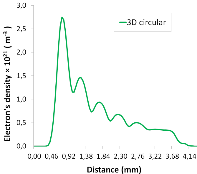
Figure 2.32: Electron density at the centerline x - axis, t = 60ns .
