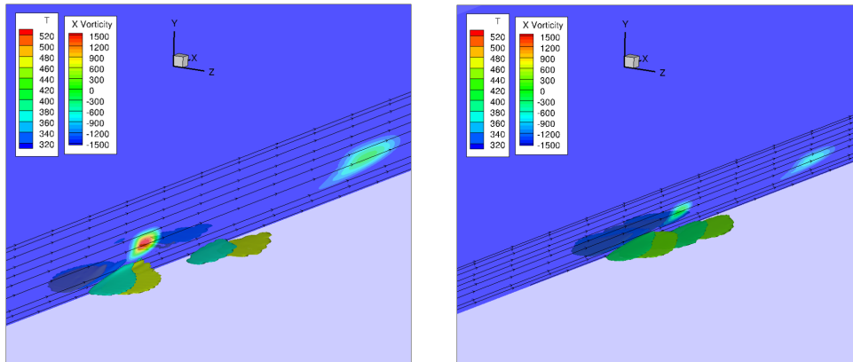
Figure 1.39: Temperature contours in the centered to the heated region xy plane and x -vorticity iso-surfaces at time t = 1.1ms and 2ms .
