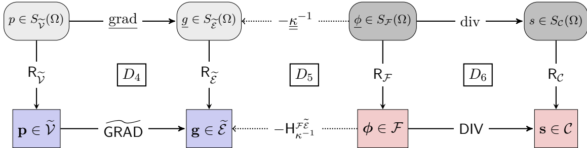
Figure 8.3 – Tonti diagrams for the exact problem and the cell-based scheme (8.34).
