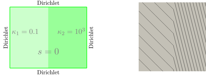
Figure 8.6 – Left: Description of the problem; Right: Isovalues of the computed potential.
