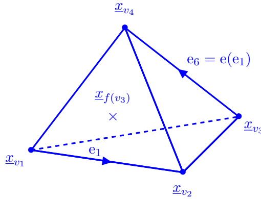
Figure 7.3 – Tetrahedron.
